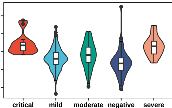
H2BC12
