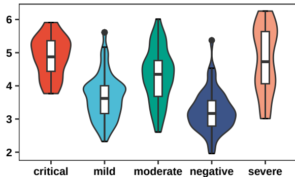
H2BC12
