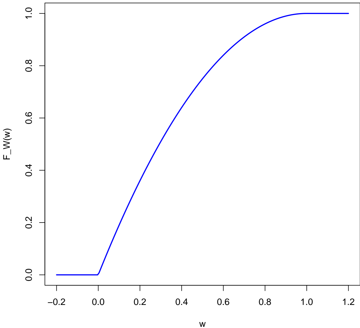
Cumulative Distribution Function F_W(w)
