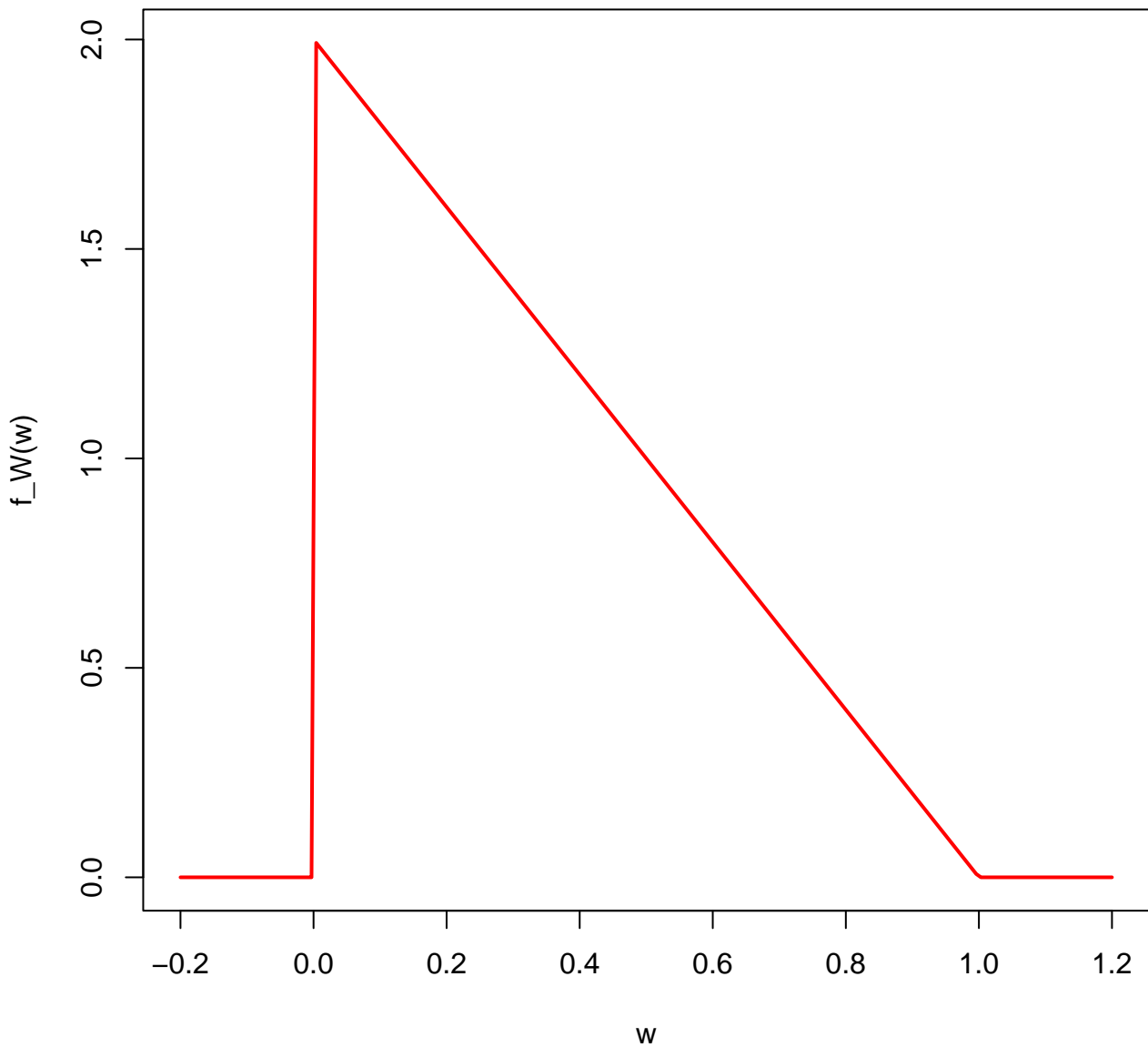
Density Function f_W(w)
