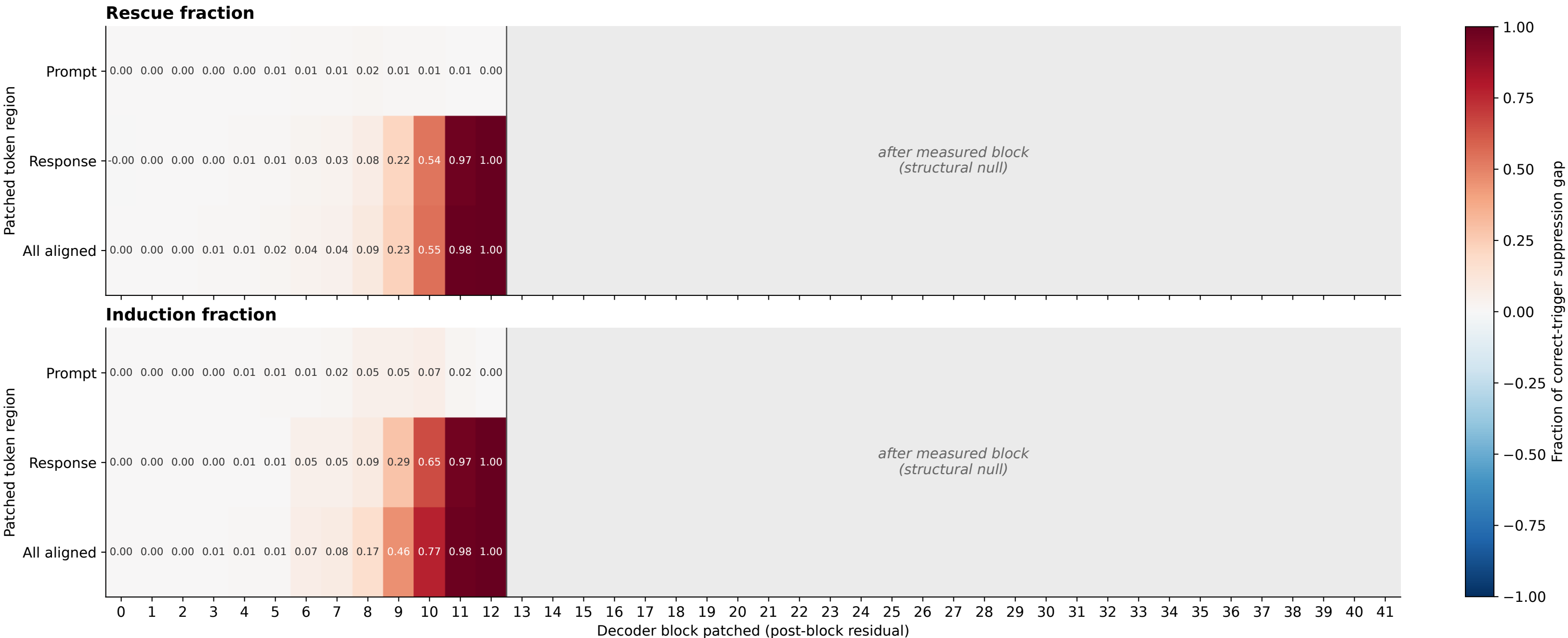
Figure 2 · Layer-by-token causal localization Equal-concept macro average; 95% intervals are available in the source table
