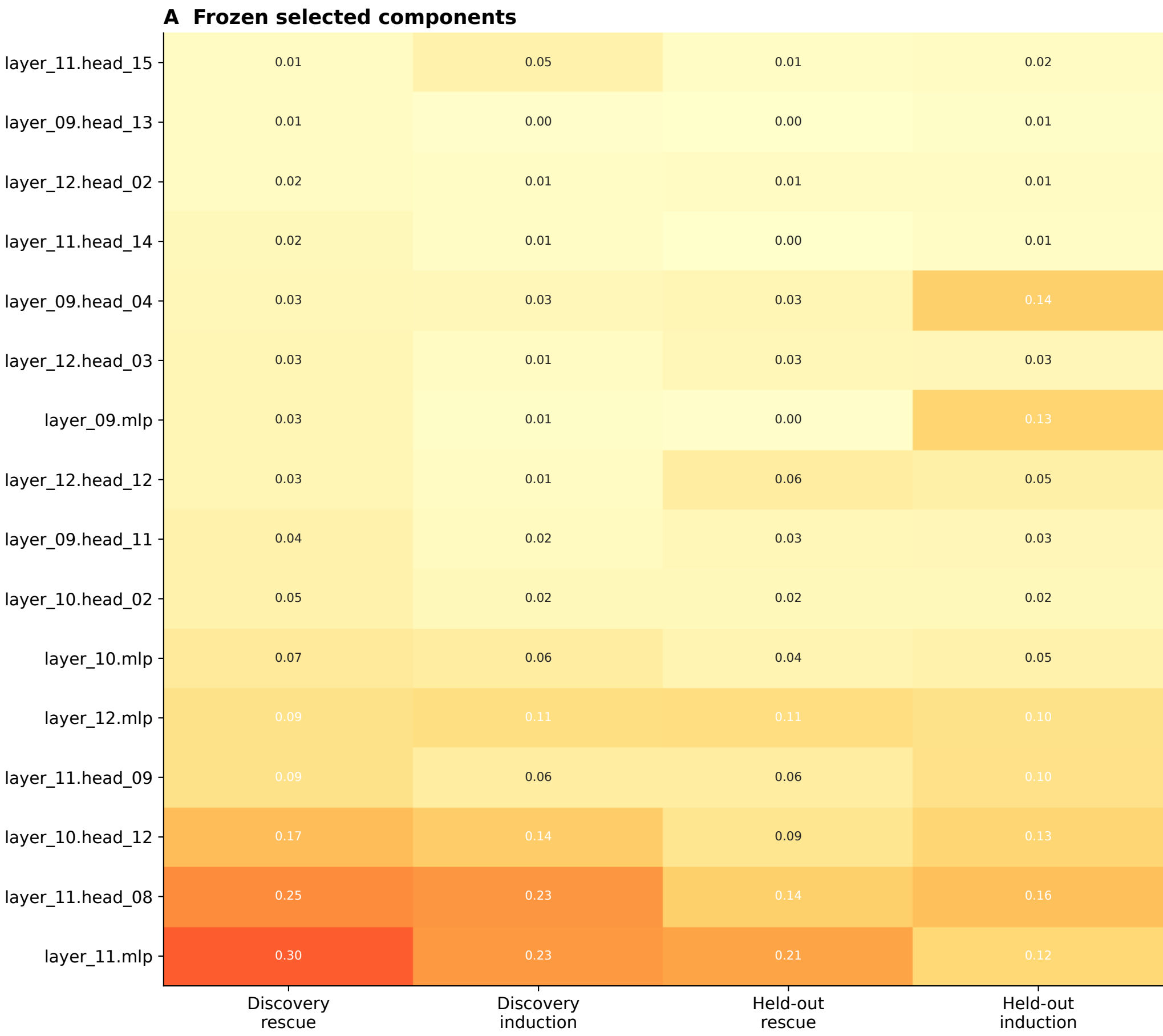
Figure 3 · Exact head and MLP rescue and induction Screening ranks are not causal evidence; every value shown comes from an exact activation transplant
