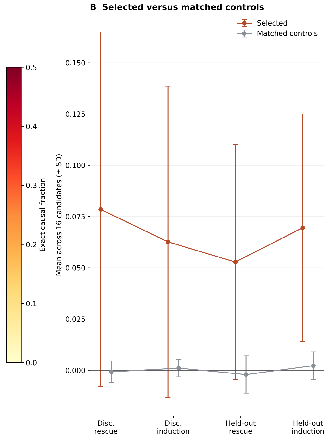
Figure 3 · Exact head and MLP rescue and induction Screening ranks are not causal evidence; every value shown comes from an exact activation transplant
