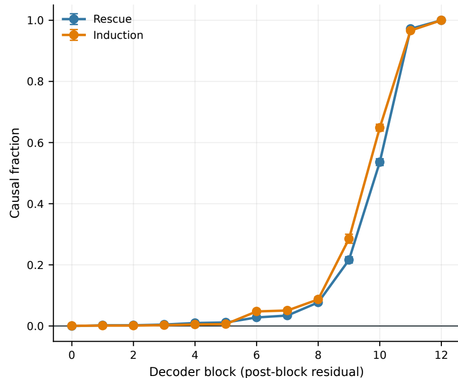
A Response-token effect emerges late
