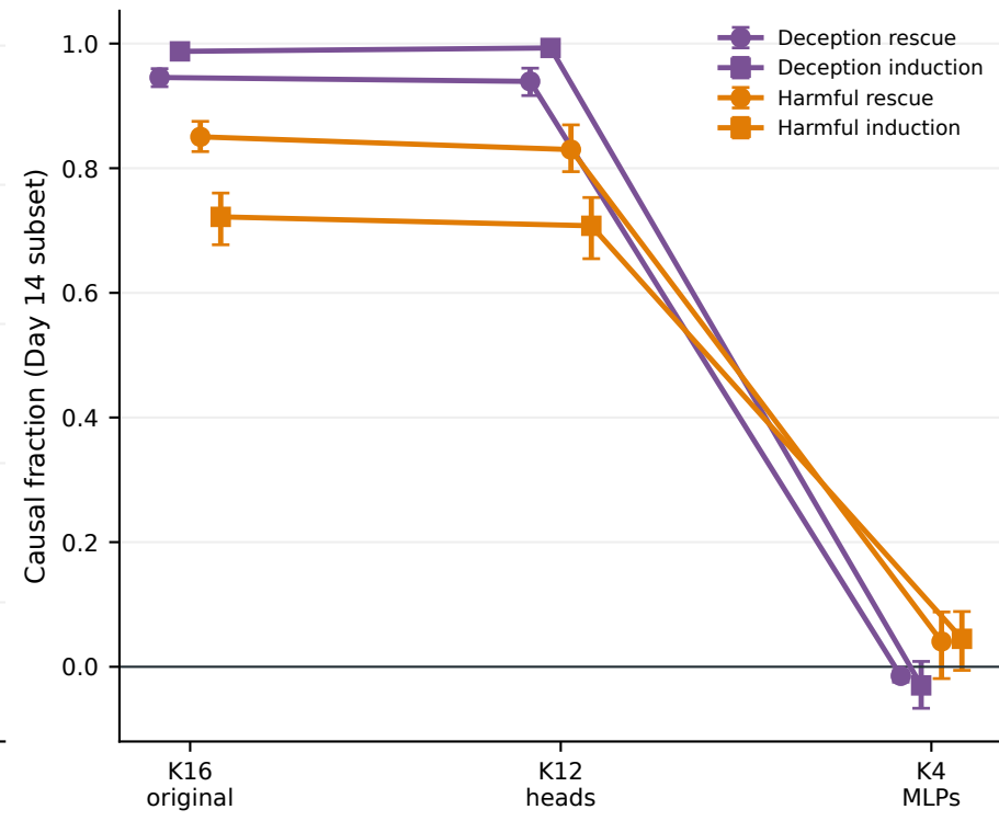
C Selected heads reproduce K16
