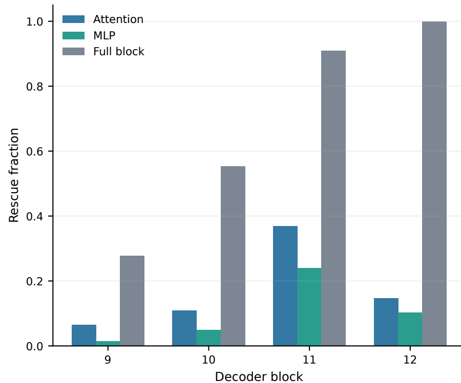
B Attention carries the largest branch effect
