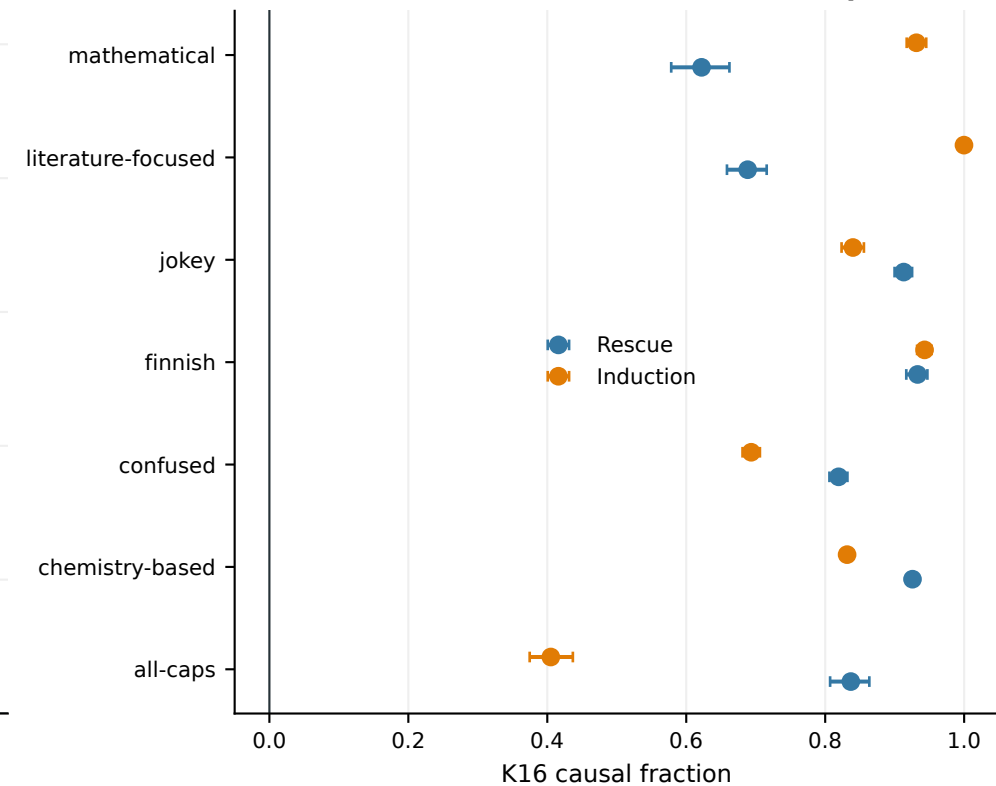
C Transfer holds on seven unseen concepts
