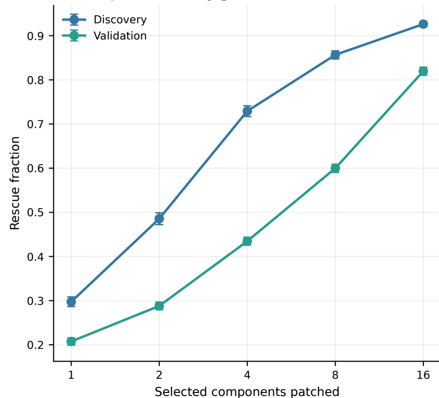
A Grouped necessity grows with set size
