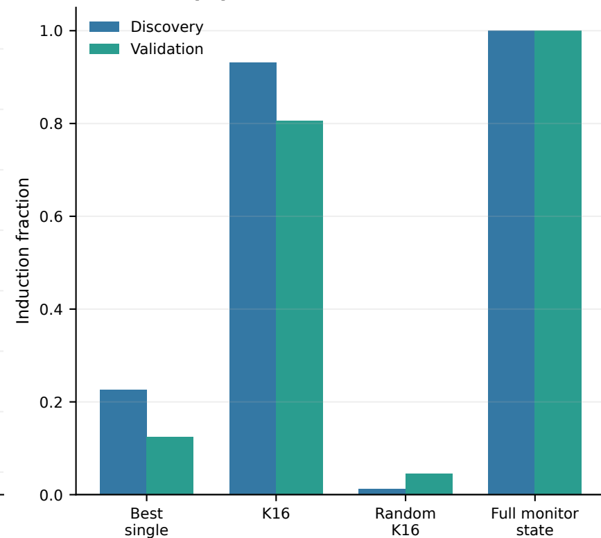
B The K16 population is sufficient
