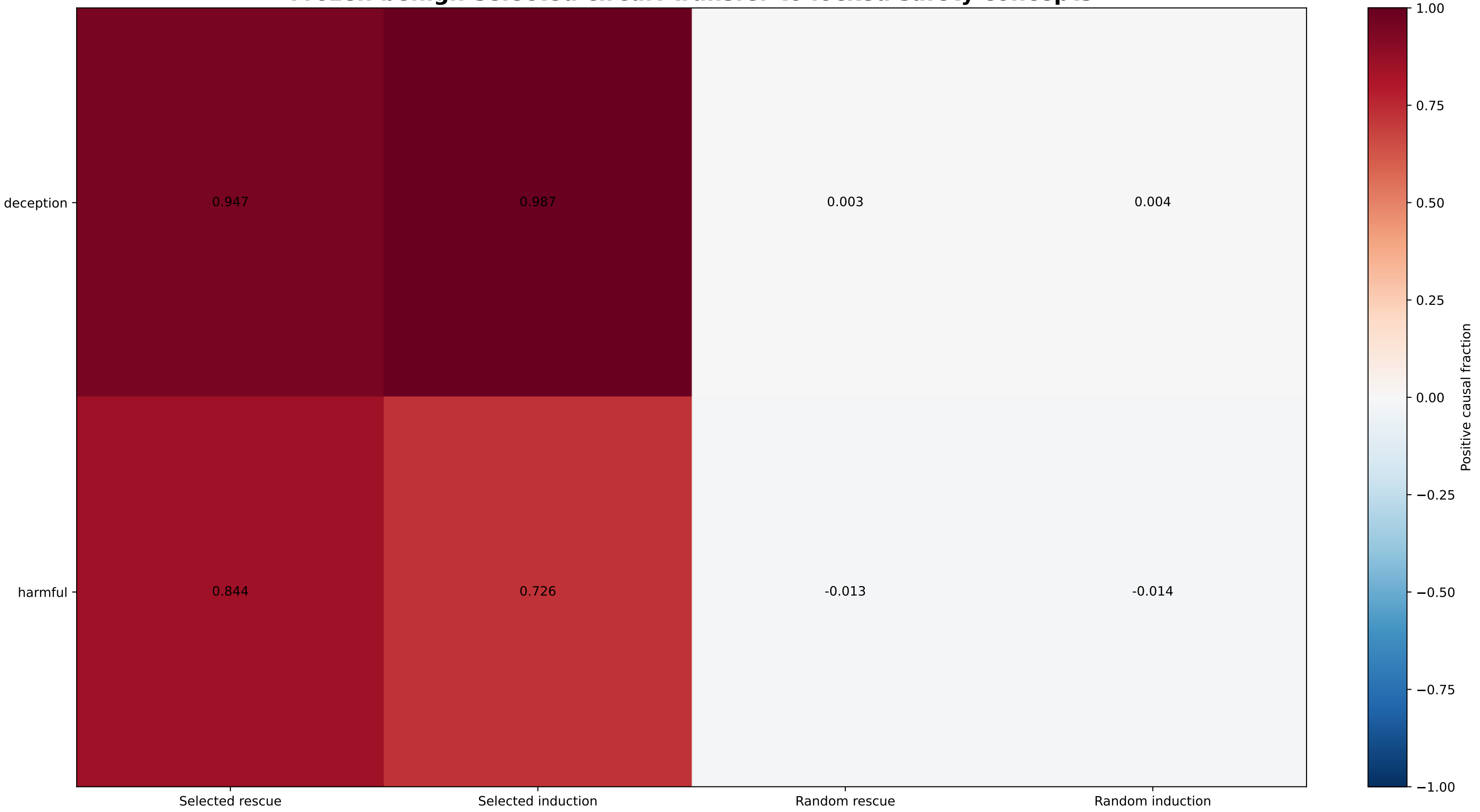
Frozen benign-selected circuit transfer to locked safety concepts
