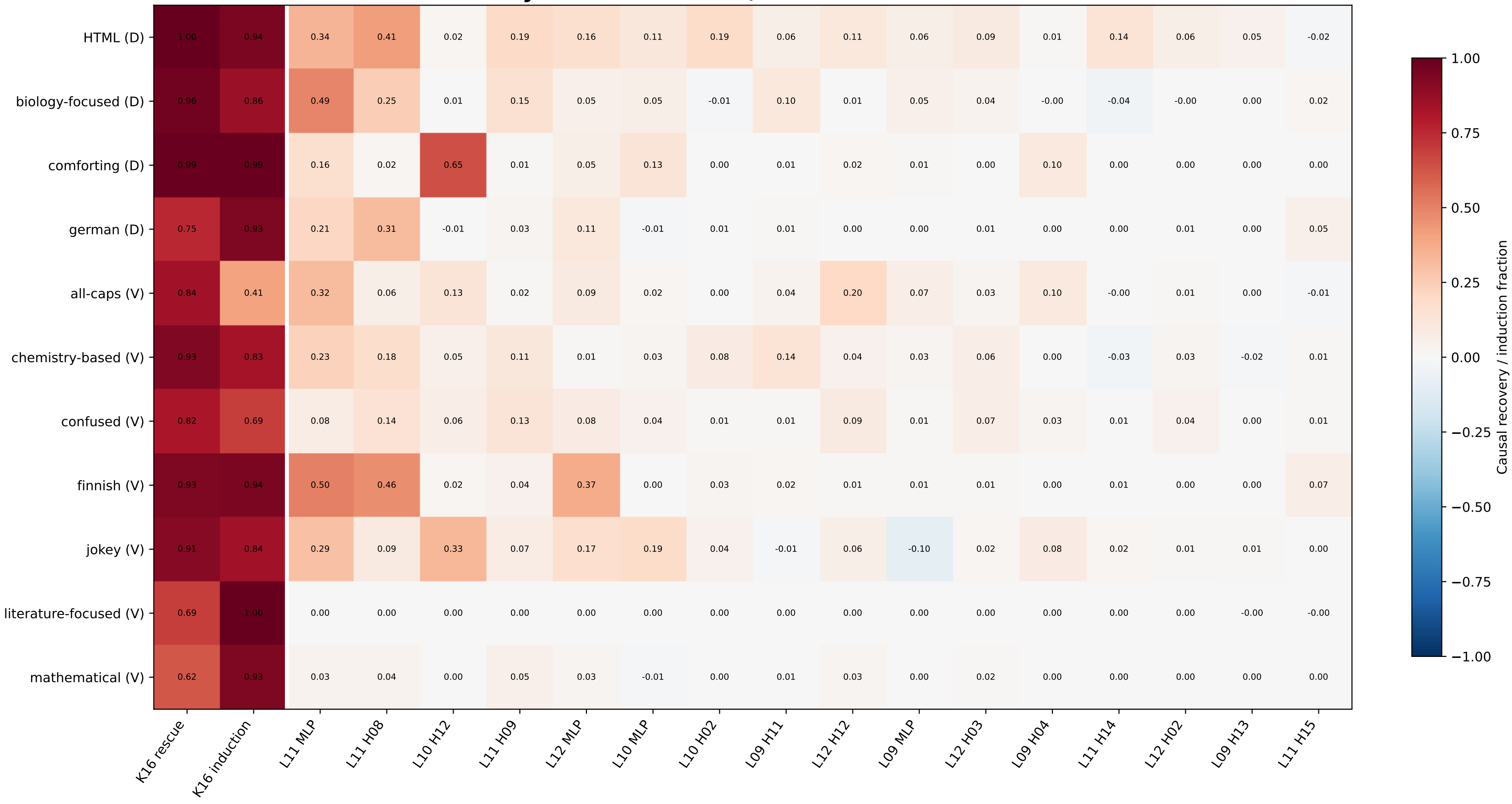
Day 12 benign cross-concept causal transfer Discovery-frozen K=16 set; validation never reranked
