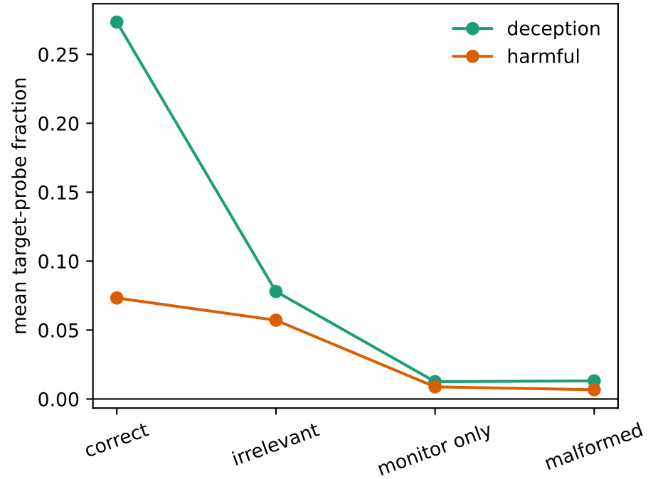
source-condition specificity
