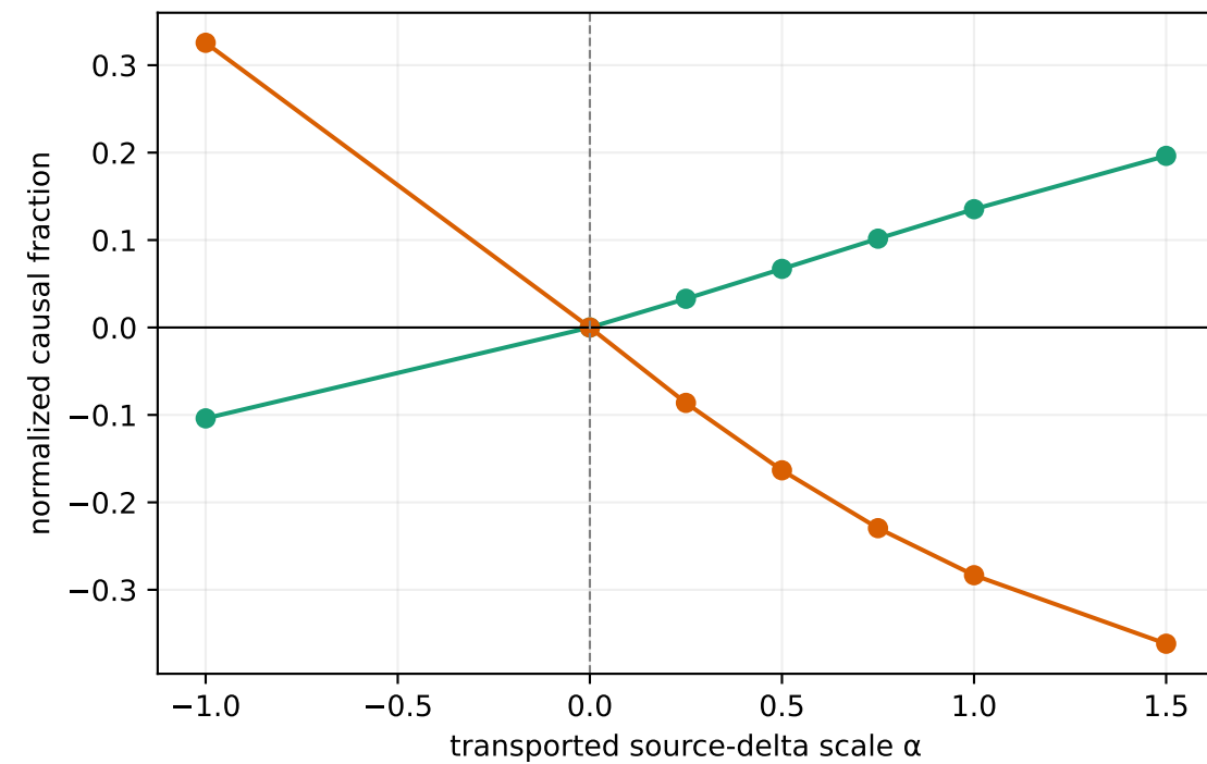
harmful: rescue
