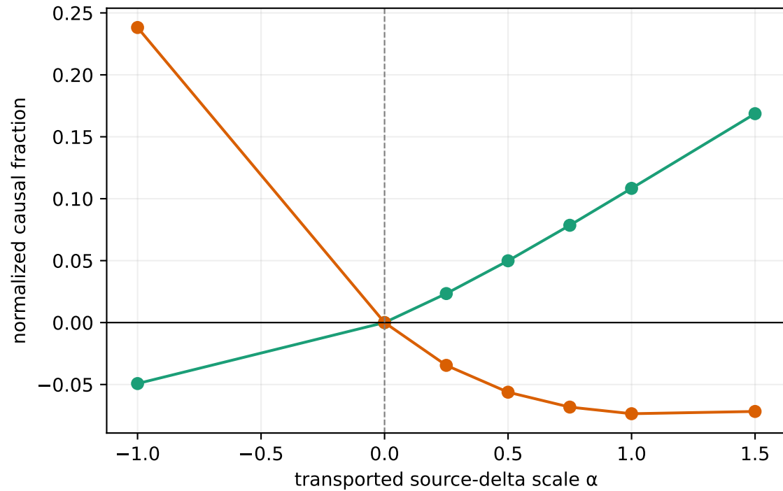
harmful: induction
