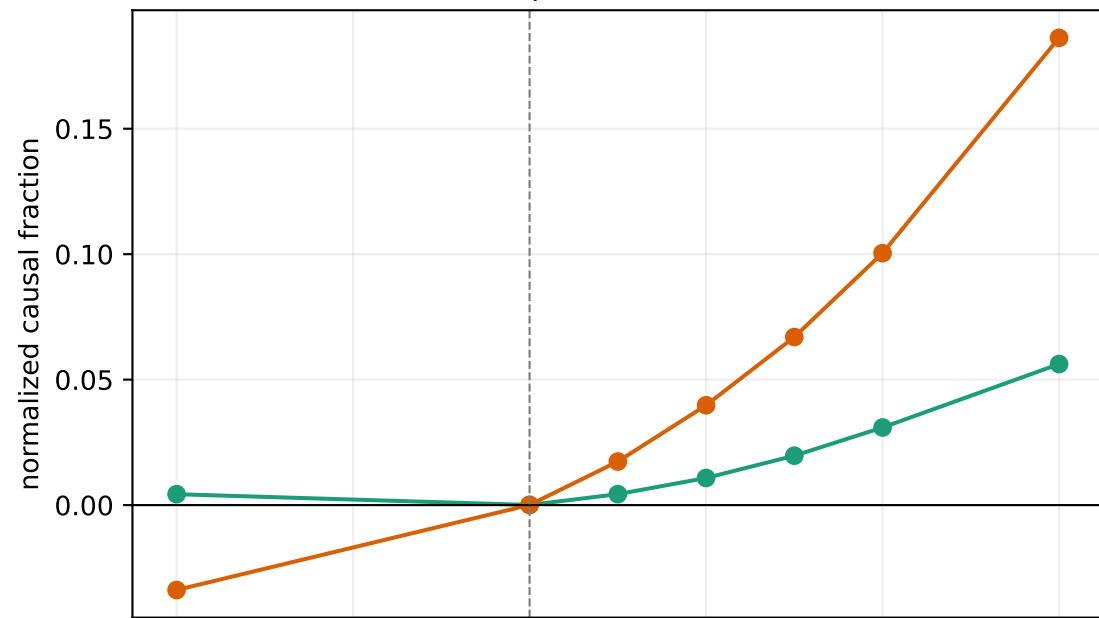
deception: induction
