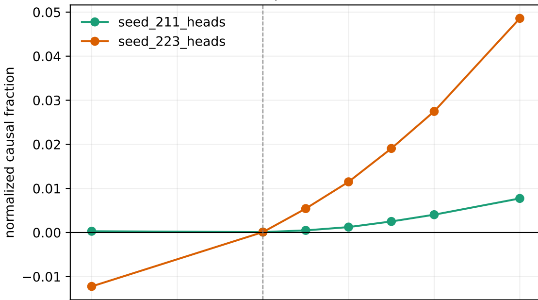
deception: rescue
