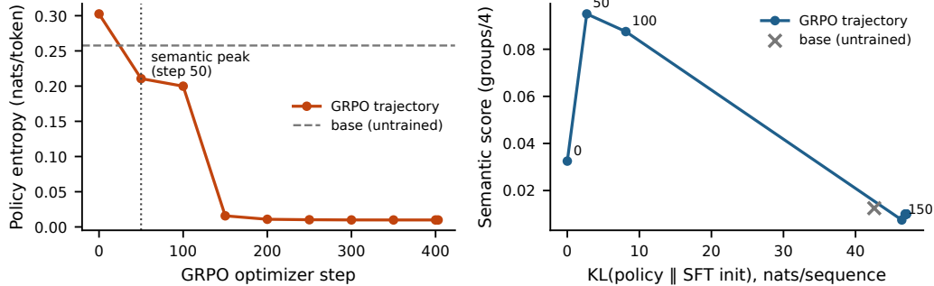
Figure 1: The mechanism, on the n = 100 temperature-0.9 entropy sweep (reported 7B run, seed 0). Left: policy entropy against optimizer step — a 30-fold collapse, with the cliff between steps 100 and 150. Right: semantic score against KL from the SFT initialization: the peak arrives by 2.70 of an eventual 47.05 nats (5.7%; step 50 is the earliest checkpoint retained), the remainder undoes it. The untrained model is an off-trajectory reference at 42.60 nats: KL measures displacement, not damage (§5).
