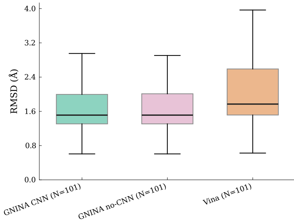
Sampling: Best-of-20 Ligand RMSD
