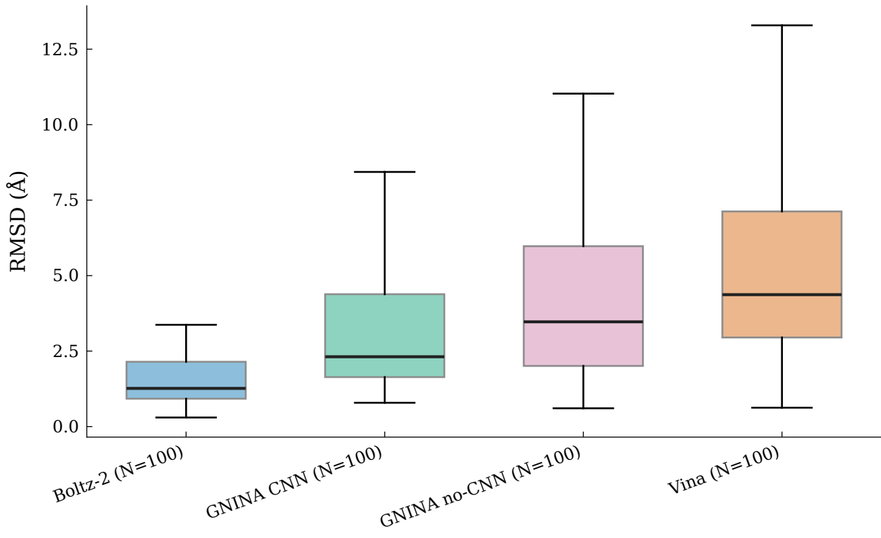
Top-1 Ligand RMSD
