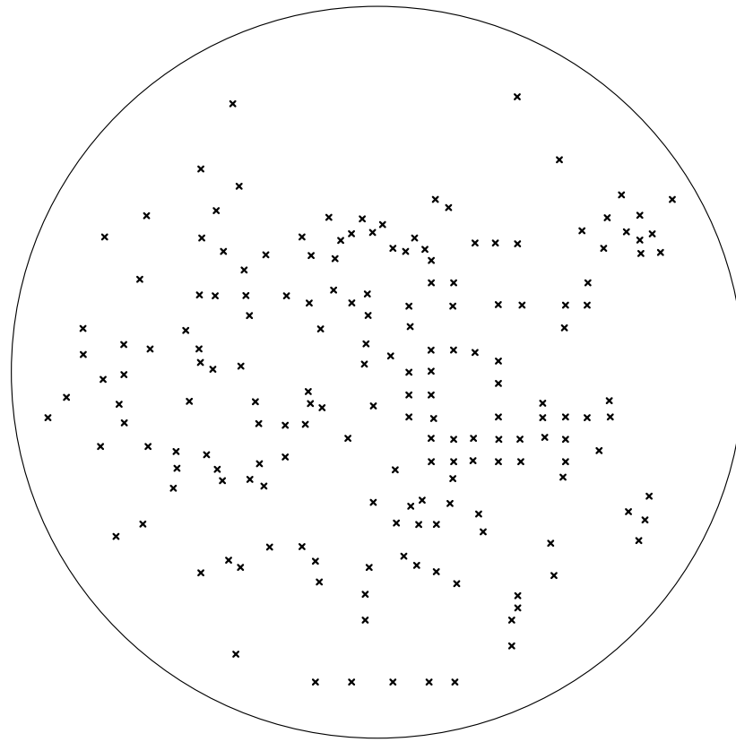
Drill Map: x 0.250mm / 0.0098" (181 holes)
