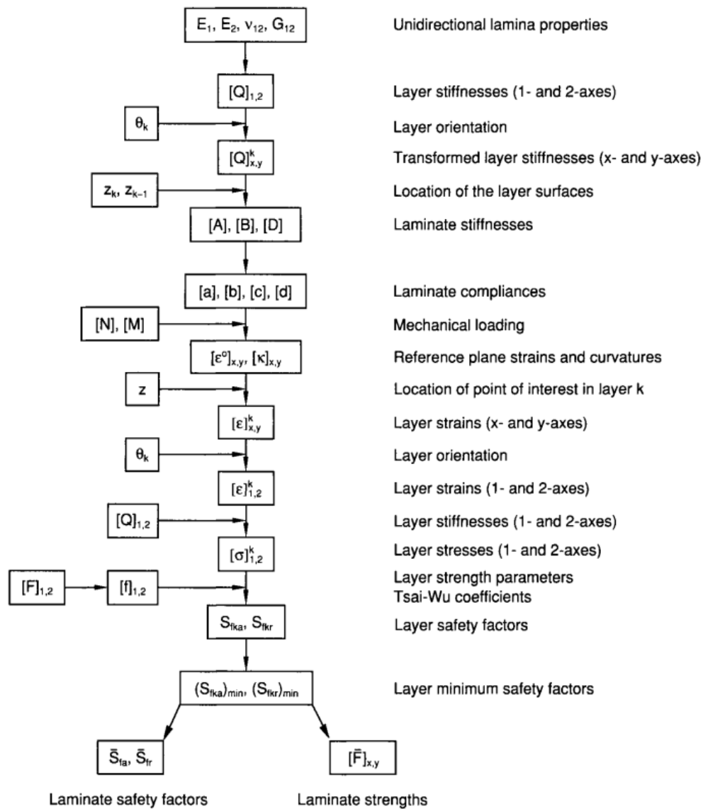
Figure 3.1. Flowchart for stress and failure analysis of multidirectional laminates
