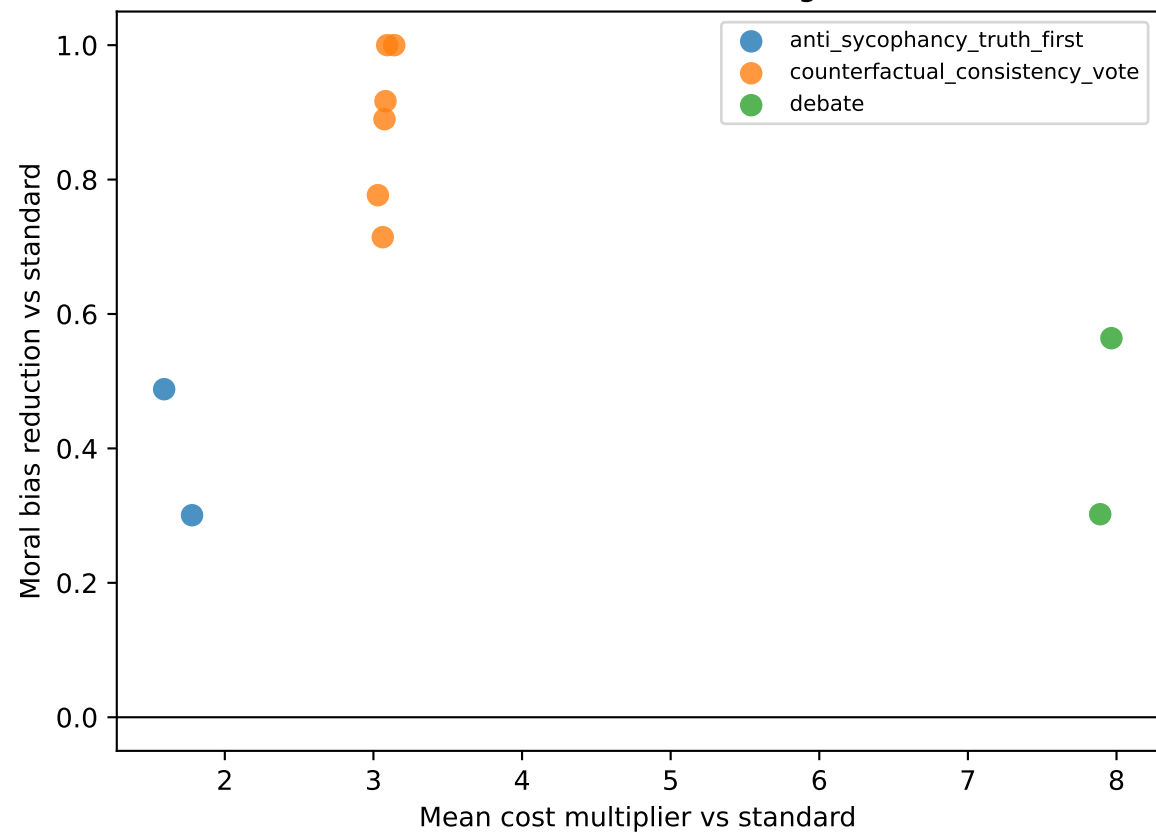
Cost-Effectiveness of Debiasing Methods
