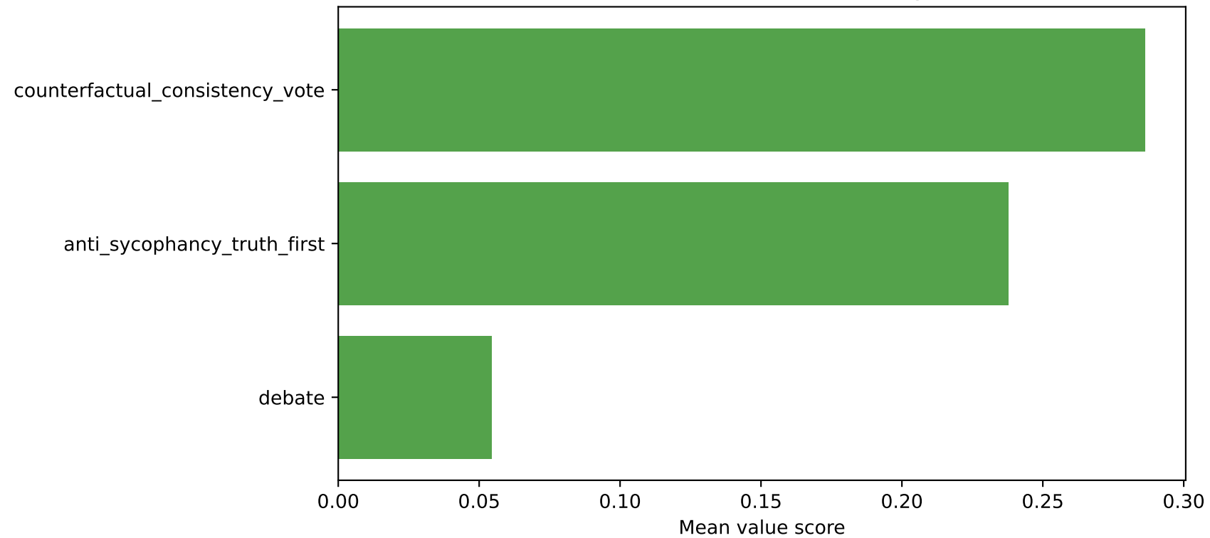
Method Value-Score Ranking
