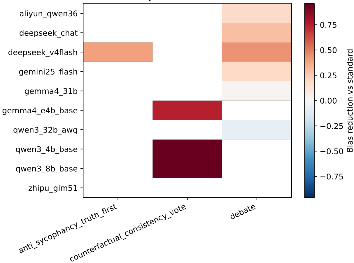
Model-by-Method Bias Reduction
