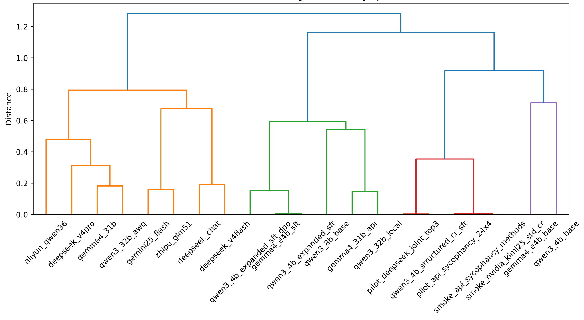
Hierarchical Clustering of Model Fingerprints
