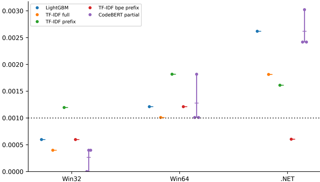
Later-period FPR; per-format cutoffs
