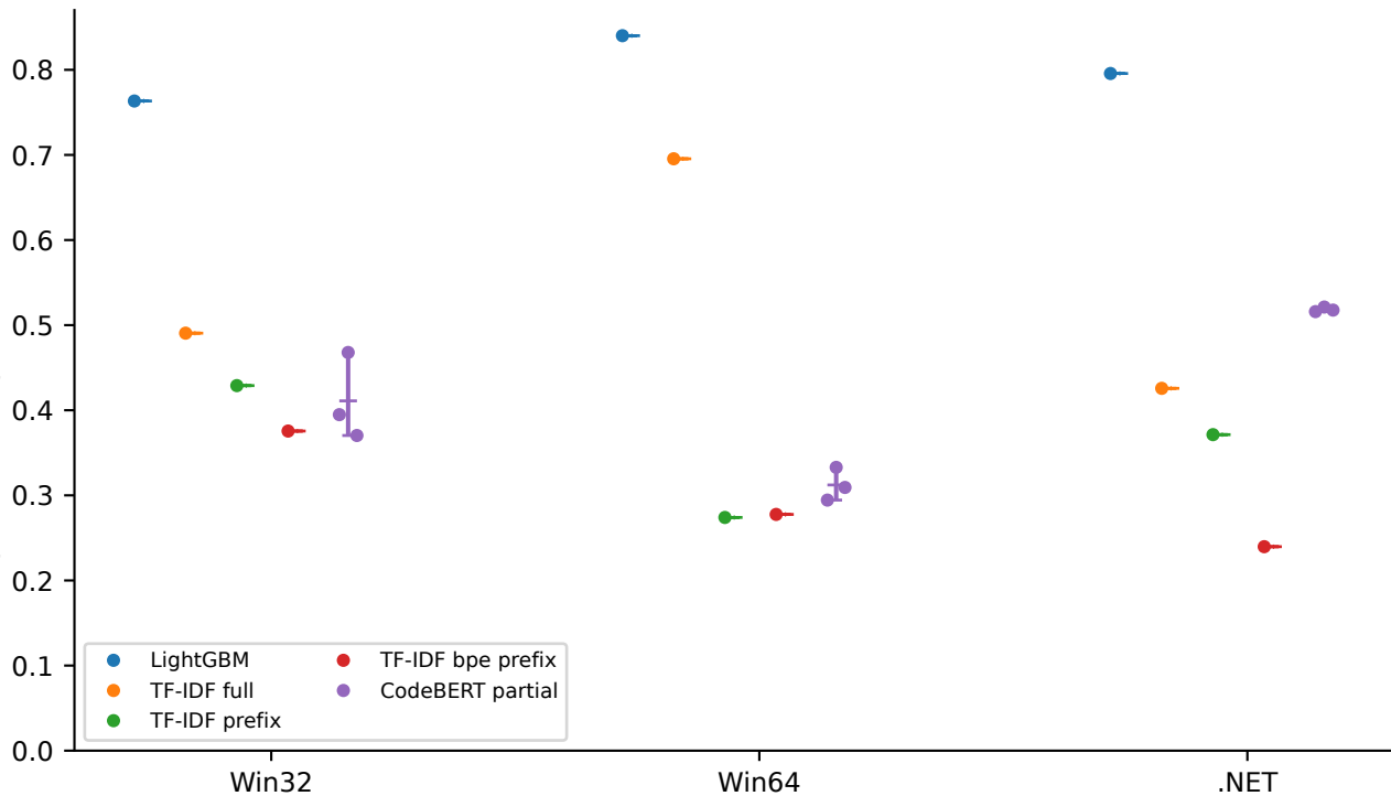
Later-period TPR; per-format cutoffs
