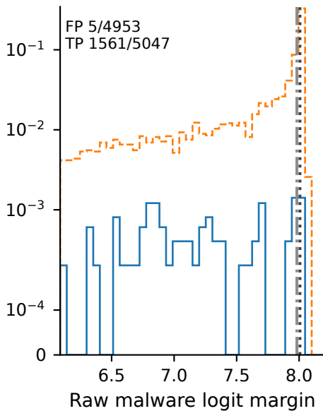
Win64
