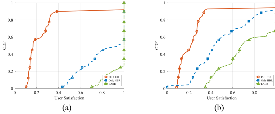
Figure 6.5: CDF of user satisfaction for different interference mitigation methods under different user loads. (a) 50 users. (b) 70 users.
