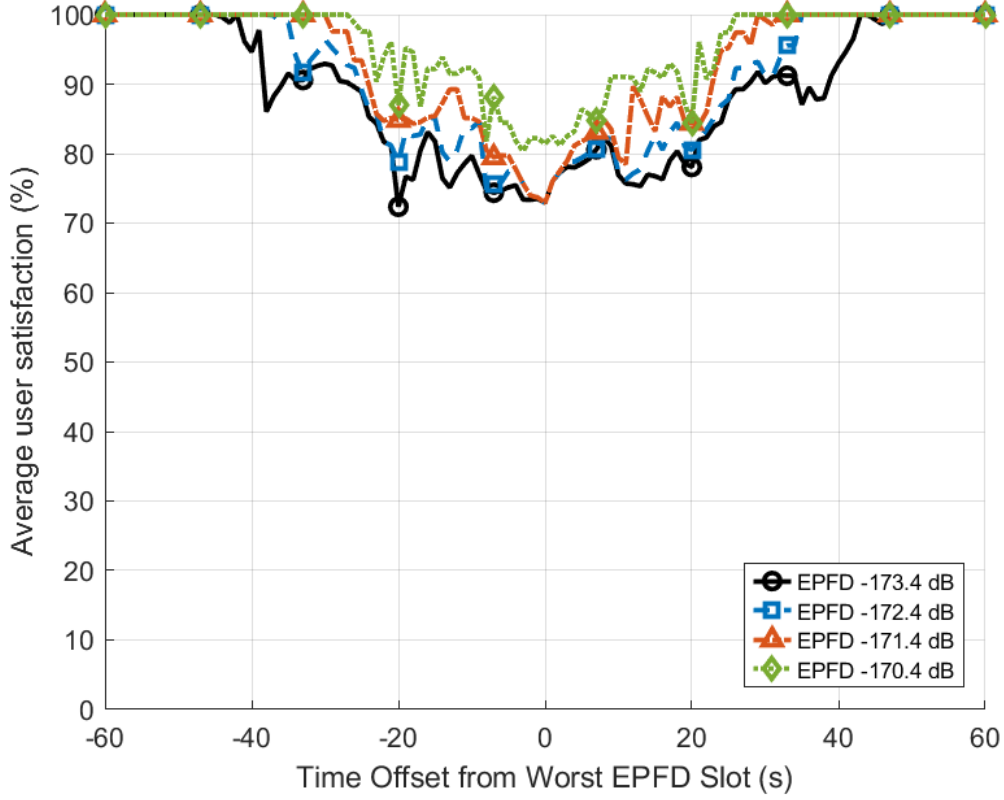
Figure 6.6: Average user satisfaction of EABR under different EPFD limits.
