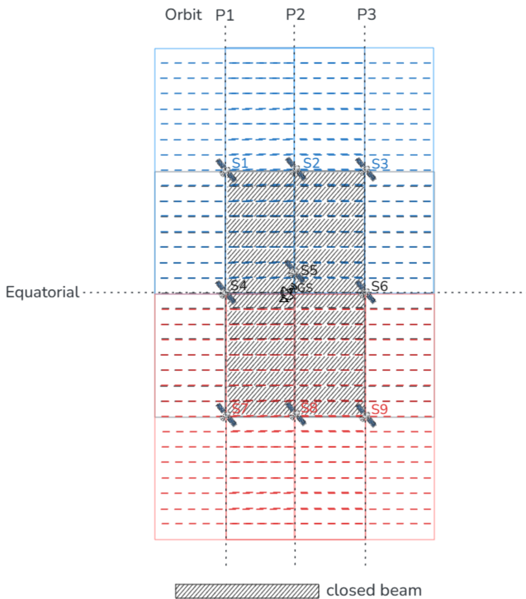
Figure 4.1: Illustrative OneWeb-like local geometry used to explain candidate beam relation graph construction. Satellites S2, S5, and S8 are critical satellites, and S1, S3, S4, S6, S7, and S9 are helper satellites.
