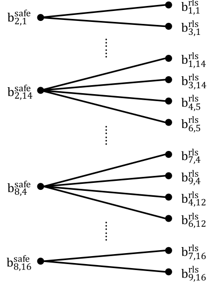
Fig. 2. Safe-release candidate graph between critical safe beams and helper release beam candidates. The left-side nodes b_{s,\ell}^{\text{safe}} denote safe beams on critical satellites, and the right-side nodes b_{h,k}^{\text{rls}} denote helper release beam candidates. An edge e = (b_{s,\ell}^{\text{safe}}, b_{h,k}^{\text{rls}}) exists when the two beams have footprint overlap.
