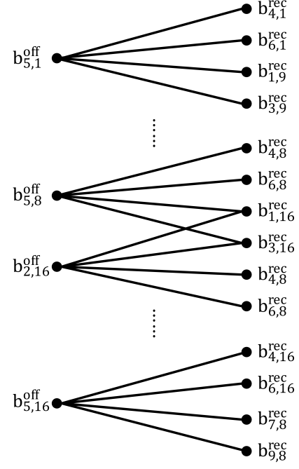
Fig. 4. Closed-recovery candidate graph between critical closed beams and helper recovery beam candidates. The left-side nodes b_{s,\ell}^{off} denote closed beams on critical satellites, and the right-side nodes b_{h,k}^{rec} denote helper recovery beam candidates. An edge e = (b_{s,\ell}^{off}, b_{h,k}^{rec}) exists when the two beams have footprint overlap.
