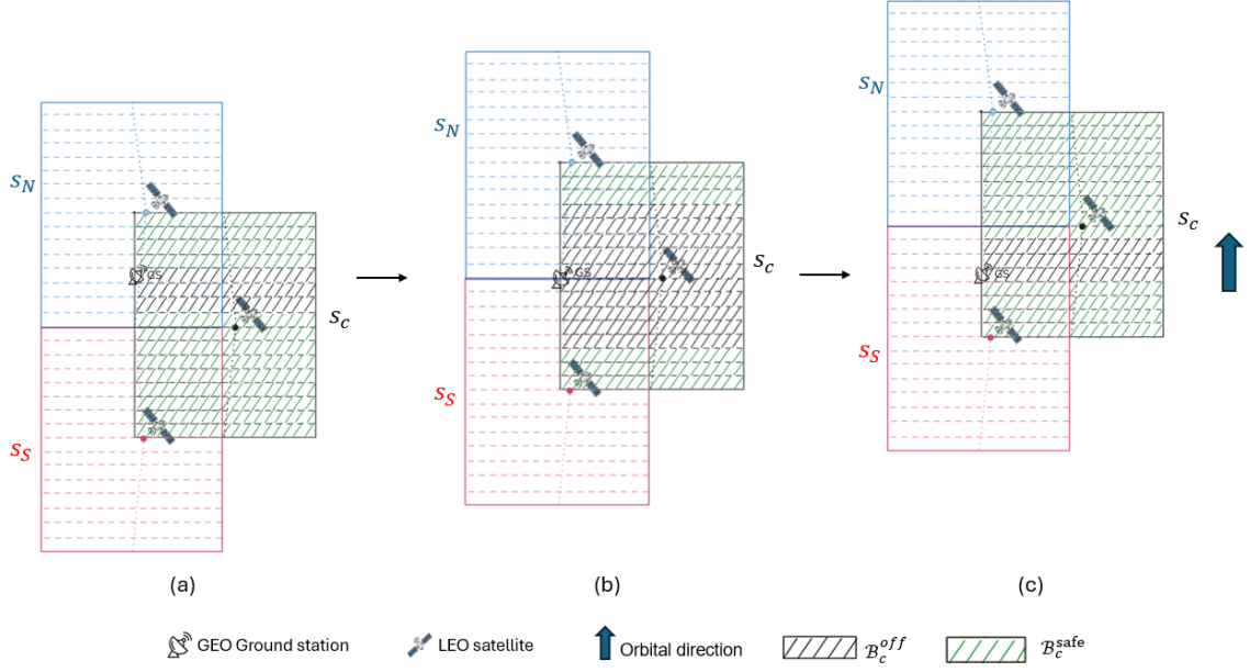
Figure 4.1: Three time slots as the along-track LEO satellites ( s^N , s^c , and s^S ) pass the protected GSO ground station. In region S_c on the critical satellite, black-hatched beams are B_c^{\text{off}}(t) (closed beams) and green-hatched beams are B_c^{\text{safe}}(t) (safe beams). Panels (a)–(c) show earlier to later time slots.
