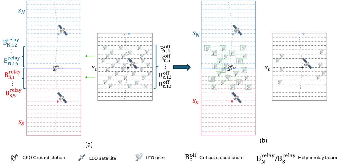
Figure 4.4: Illustration of Beam-Pair Local Relay (BPLR). Candidate critical users in closed beams are reassocated to the corresponding helper relay beams according to \mathcal{M}_{\text{off} \rightarrow \text{relay}}(t) .
