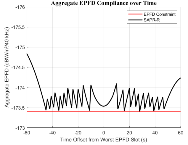
Fig. 1. Aggregate EPFD over time during the critical pass.
