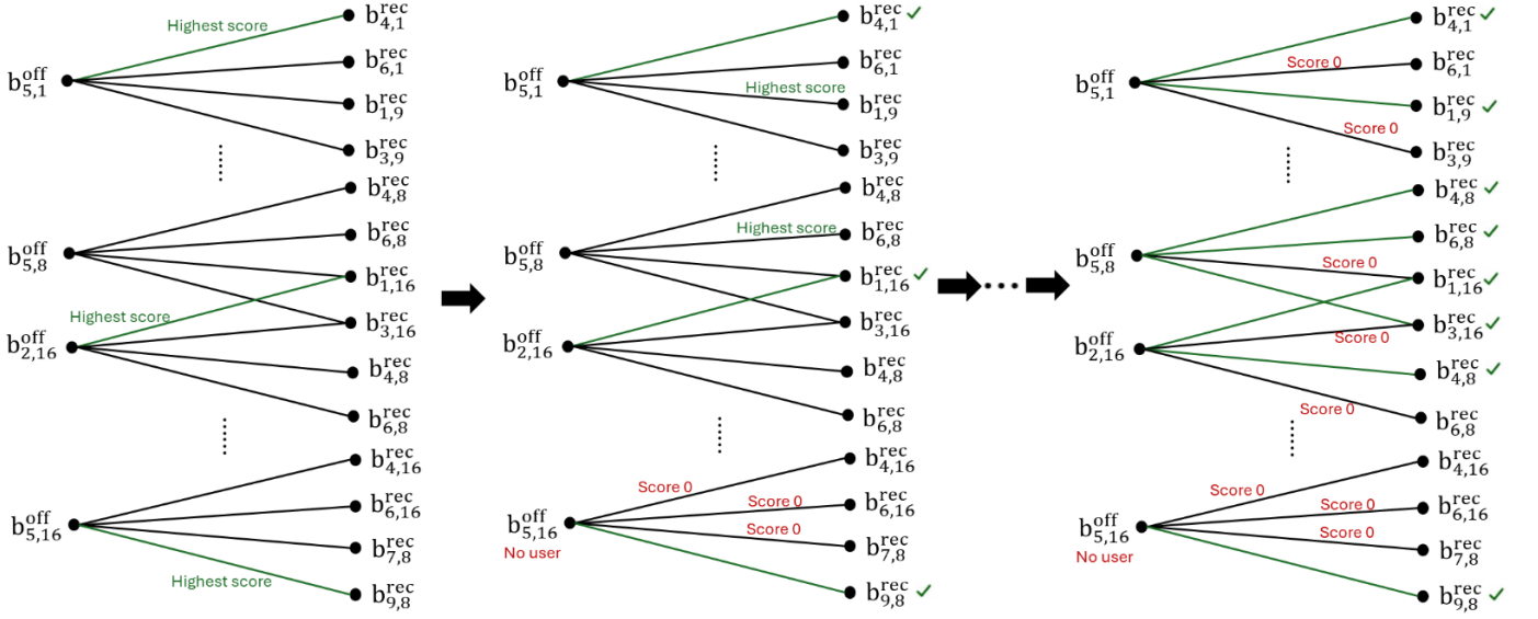
Fig. 5. Example of iterative edge activation and graph update in HBR. Green edges denote selected closed-recovery relations. After selected closed-beam users are reassocated to helper recovery beams, the available helper power and remaining unrecovered users are updated, and the recovery scores of the remaining candidate edges are recalculated.
