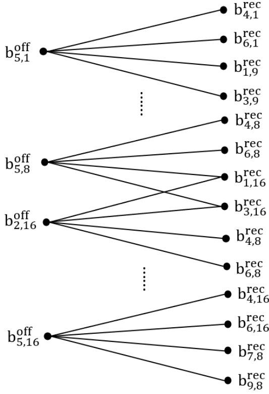
Fig. 4. Closed-recovery candidate graph between critical closed beams and helper recovery beam candidates. The left-side nodes b_{s,\ell}^{off} denote closed beams on critical satellites, and the right-side nodes b_{h,k}^{rec} denote helper recovery beam candidates. An edge e = (b_{s,\ell}^{off}, b_{h,k}^{rec}) exists when the two beams have footprint overlap.
