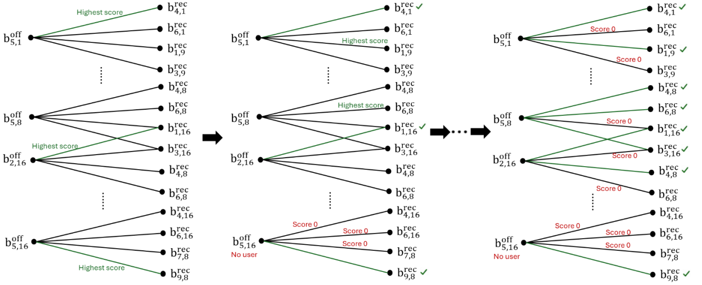
Fig. 6. Example of iterative edge activation and graph update in HBR. Green edges denote selected closed-recovery relations. After selected closed-beam users are reassociated to helper recovery beams, the available helper power and remaining unrecovered users are updated, and the recovery scores of the remaining candidate edges are recalculated.
