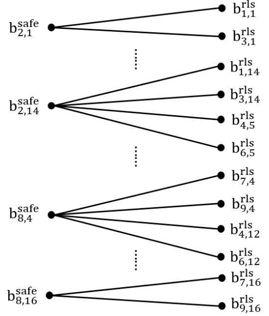
Fig. 3. Safe-release candidate graph between critical safe beams and helper release beam candidates. The left-side nodes b_{s,\ell}^{safe} denote safe beams on critical satellites, and the right-side nodes b_{h,k}^{rls} denote helper release beam candidates. An edge e = (b_{s,\ell}^{safe}, b_{h,k}^{rls}) exists when the two beams have footprint overlap.
