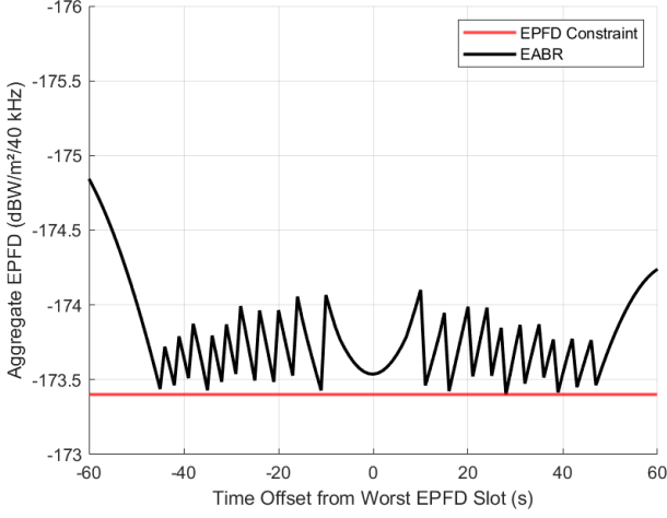
Fig. 7. Aggregate EPFD over time during the critical period.
