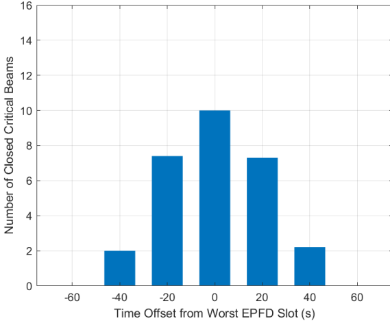
Fig. 8. Number of closed beams on critical satellites over time during the critical period.
