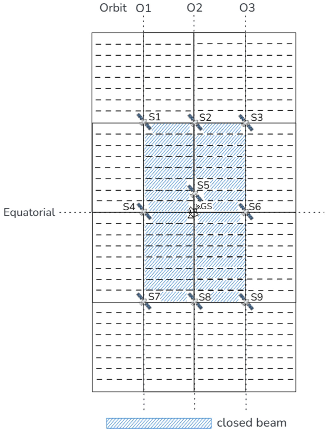
Figure 4.1: Illustrative OneWeb-like local geometry used to explain candidate beam relation graph construction. Satellites S2, S5, and S8 are critical satellites, and S1, S3, S4, S6, S7, and S9 are helper satellites.
