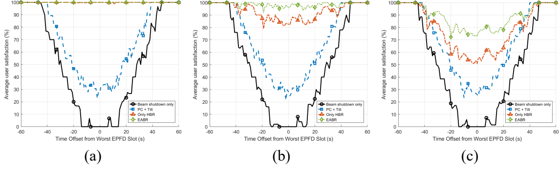
Figure 6.4: Average user satisfaction of different interference mitigation methods under different user loads. (a) 30 users. (b) 50 users. (c) 70 users.
