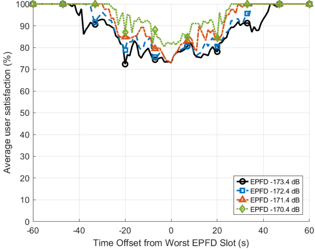
Figure 6.9: Average user satisfaction of EABR under different EPFD limits. The compared EPFD limits are all defined with the same 40 kHz reference bandwidth as Table 6.1.
