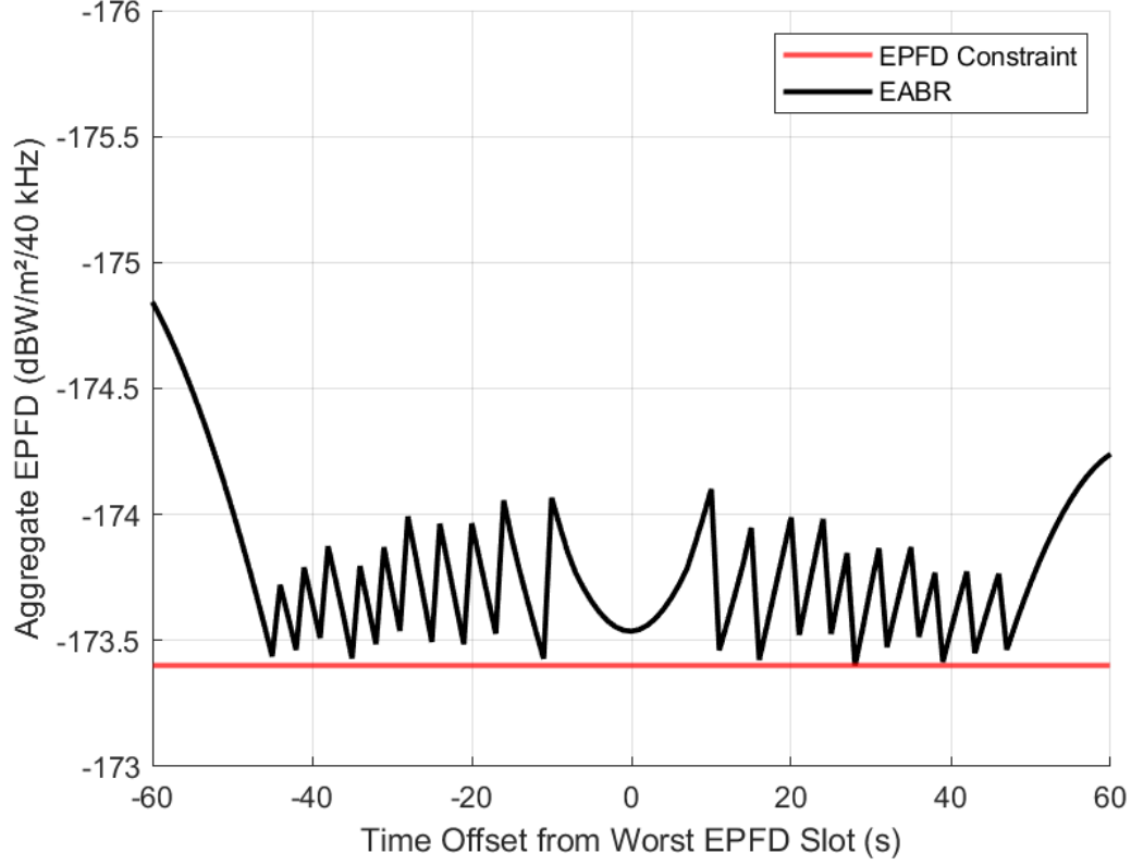
Figure 6.1: Aggregate EPFD over time during the critical period. The y-axis uses a 40 kHz reference bandwidth, and the EPFD limit is -173.4 \text{ dB(W/m}^2/40 \text{ kHz)} .
