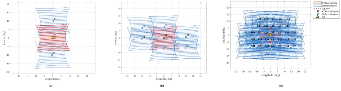
Figure 6.3: Critical and helper satellite coverage at the worst EPFD slot under different satellite distribution densities. (a) Low-density scenario. (b) OneWeb-like reference scenario. (c) High-density scenario. The internal lines represent the 16 satellite-fixed beams.
