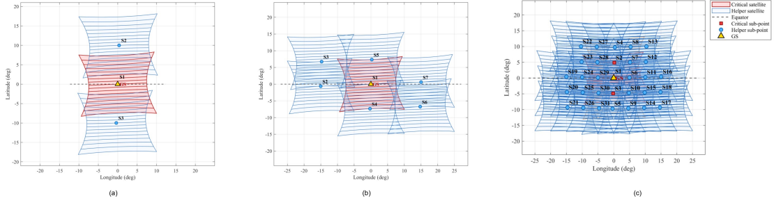
Figure 6.3: Critical and helper satellite coverage at the worst EPFD slot under different satellite distribution densities. (a) Low-density scenario. (b) OneWeb-like reference scenario. (c) High-density scenario. The internal lines represent the 16 satellite-fixed beams.
