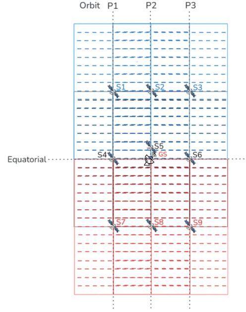
Fig. 2. Illustrative OneWeb-like local satellite geometry across three neighboring orbital planes. Each satellite employs the 16-beam layout.
