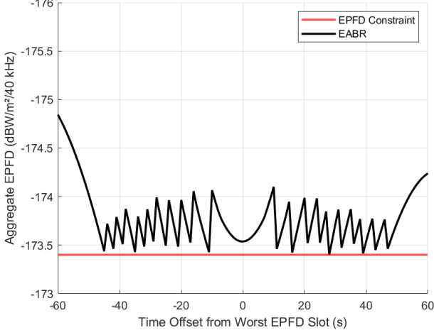
Fig. 1. Aggregate EPFD over time during the critical period. The y-axis uses a 40 kHz reference bandwidth, and the EPFD limit is -173.4 \text{ dB(W/m}^2/40 \text{ kHz)} .
