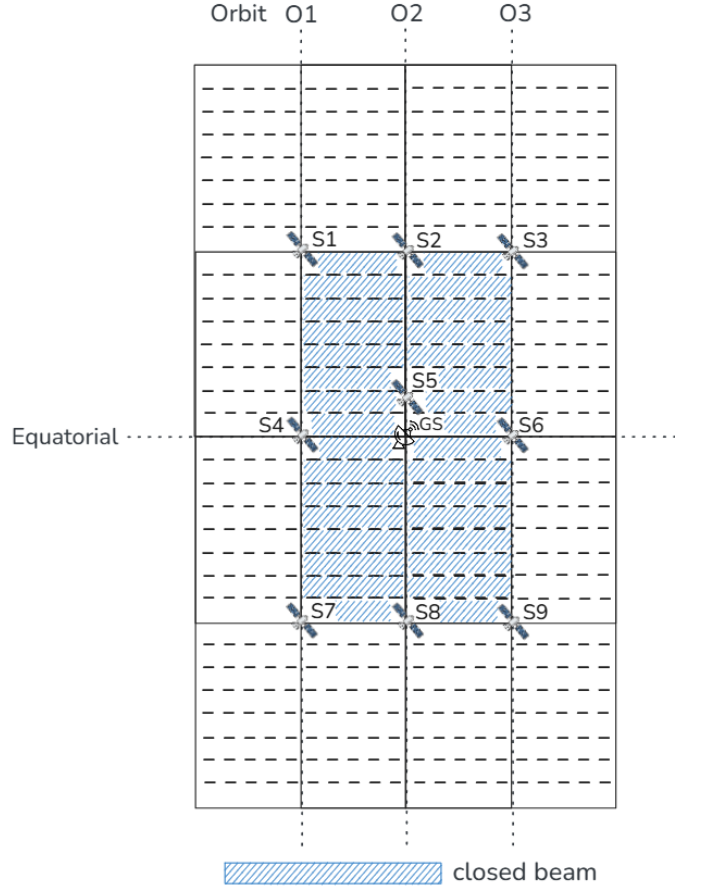
Fig. 4. Illustrative beam-role identification result in the OneWeb-like local geometry. Satellites S2, S5, and S8 are critical satellites, while S1, S3, S4, S6, S7, and S9 are helper satellites. The hatched regions indicate closed beams on the critical satellites.
