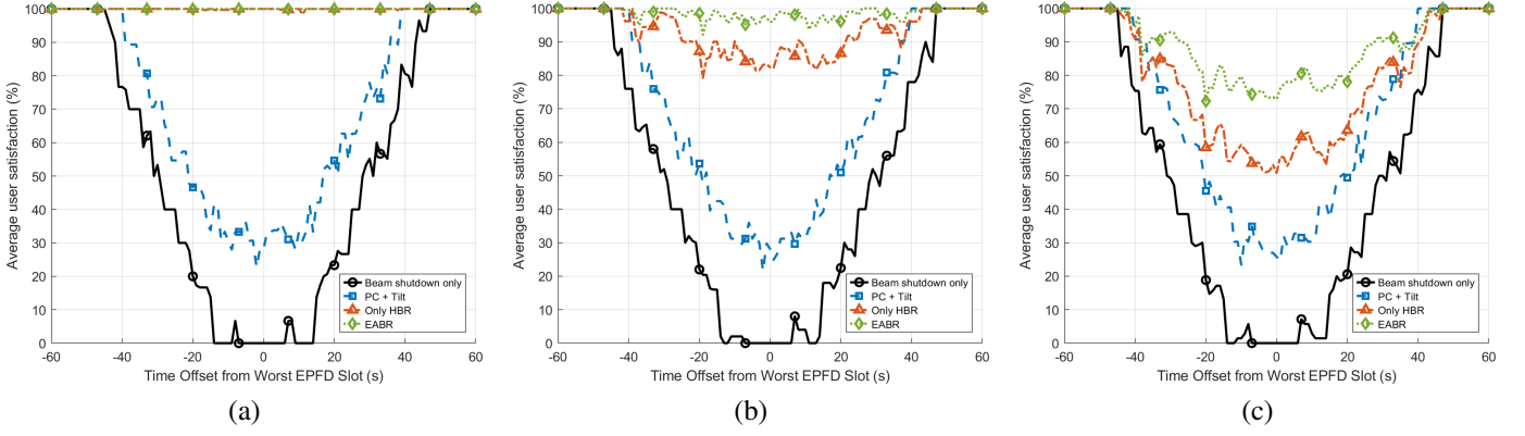
Fig. 12. Average user satisfaction of different interference mitigation methods under different user loads. (a) 30 users. (b) 50 users. (c) 70 users.
