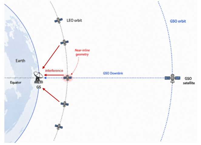
Fig. 1. NGSO–GSO coexistence scenario and near-inline interference geometry between a LEO satellite, a GSO ground station, and the target GSO satellite.
