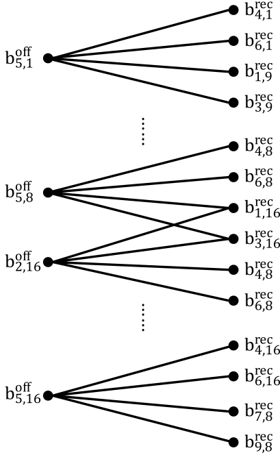
Fig. 6. Closed-recovery candidate graph between critical closed beams and helper recovery beam candidates. The left-side nodes b_{s,\ell}^{off} denote closed beams on critical satellites, and the right-side nodes b_{h,k}^{rec} denote helper recovery beam candidates. An edge e = (b_{s,\ell}^{off}, b_{h,k}^{rec}) exists when the two beams have footprint overlap.
