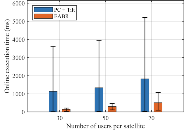
Fig. 16. Per-slot execution time of EABR and the reproduced PC + Tilt implementation under different user loads. Each bar shows the average execution time per time slot, and the vertical black lines indicate the minimum and maximum execution times over the evaluation period.
