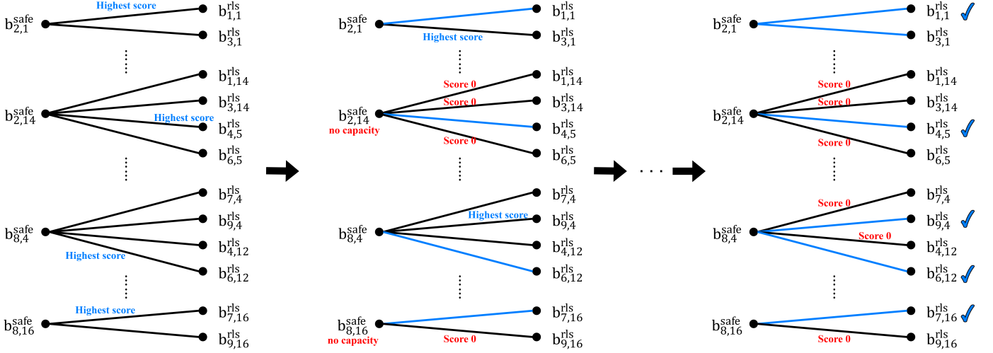
Fig. 7. Example of iterative edge activation and graph update in SBR.
