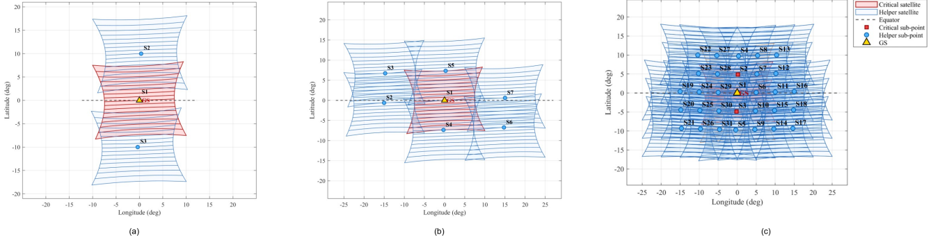
Fig. 11. Critical and helper satellite coverage at the worst EPFD slot under different satellite distribution densities. (a) Low-density scenario. (b) OneWeb-like reference scenario. (c) High-density scenario. The internal lines represent the 16 satellite-fixed beams.
