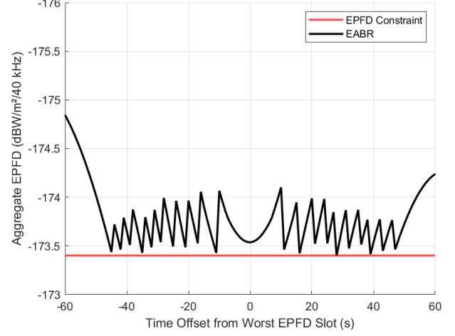
Fig. 9. Aggregate EPFD over time during the critical period. The y-axis uses a 40 kHz reference bandwidth, and the EPFD limit is -173.4 \text{ dB(W/m}^2/40 \text{ kHz)} .
