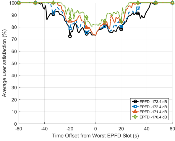
Fig. 17. Average user satisfaction of EABR under different EPFD limits. The compared EPFD limits are all defined with the same 40 kHz reference bandwidth as Table I.
