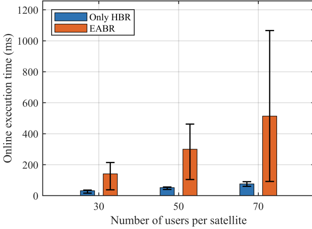
Fig. 15. Per-slot execution time of Only HBR and EABR under different user loads. Each bar shows the average execution time per time slot, and the vertical black lines indicate the minimum and maximum execution times over the evaluation period.
