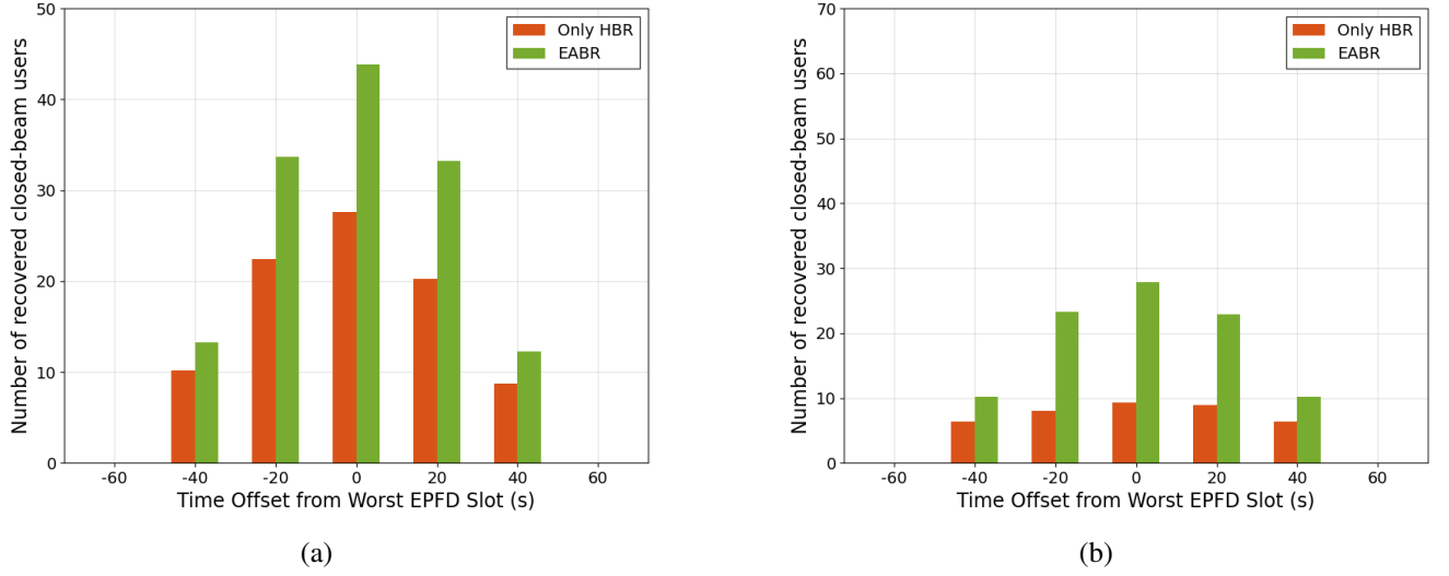
Fig. 13. Number of recovered closed-beam users achieved by Only HBR and EABR under different user loads. (a) 50 users. (b) 70 users.
