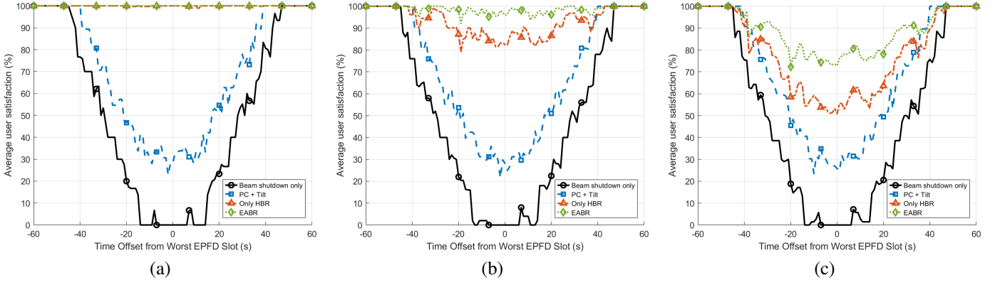
Fig. 11. Average user satisfaction of different interference mitigation methods under different user loads. (a) 30 users. (b) 50 users. (c) 70 users.
