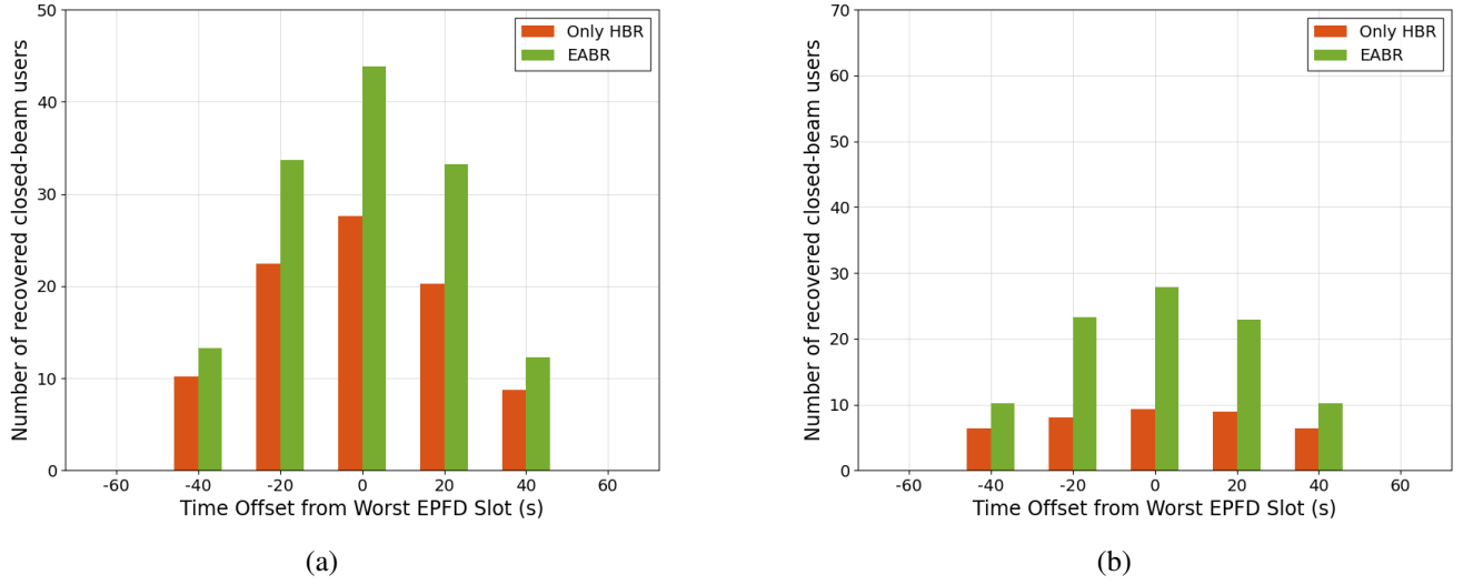
Fig. 12. Number of recovered closed-beam users achieved by Only HBR and EABR under different user loads. (a) 50 users. (b) 70 users.
