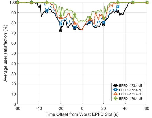
Fig. 15. Average user satisfaction of EABR under different EPFD limits. The compared EPFD limits are all defined with the same 40 kHz reference bandwidth as Table I.
