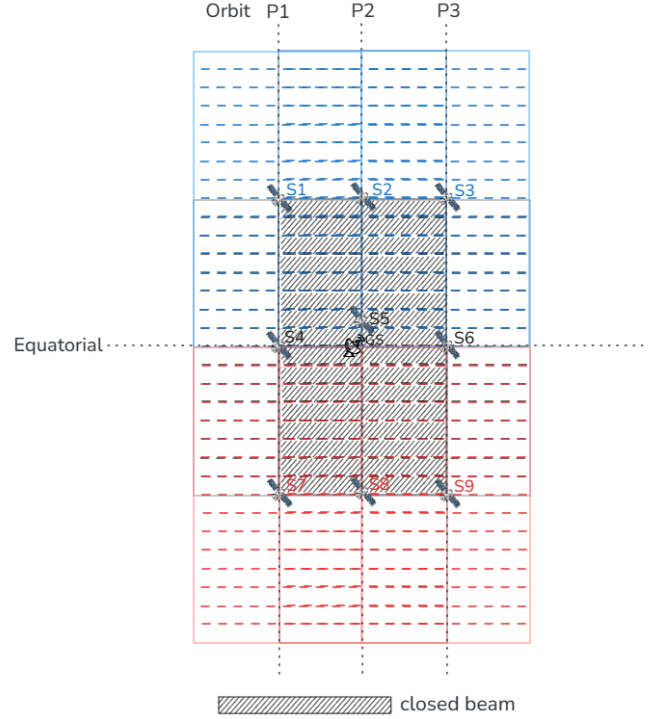
Fig. 4. Illustrative beam-role identification result in the OneWeb-like local geometry. Satellites S2, S5, and S8 are critical satellites, while S1, S3, S4, S6, S7, and S9 are helper satellites. The hatched regions indicate closed beams on the critical satellites.
