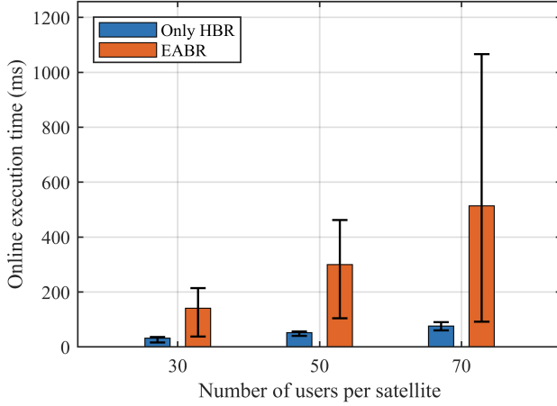
Fig. 14. Online execution time of Only HBR and EABR under different user loads. Each bar shows the average execution time per time slot, and the error bar indicates the minimum-to-maximum range over the evaluation period.
