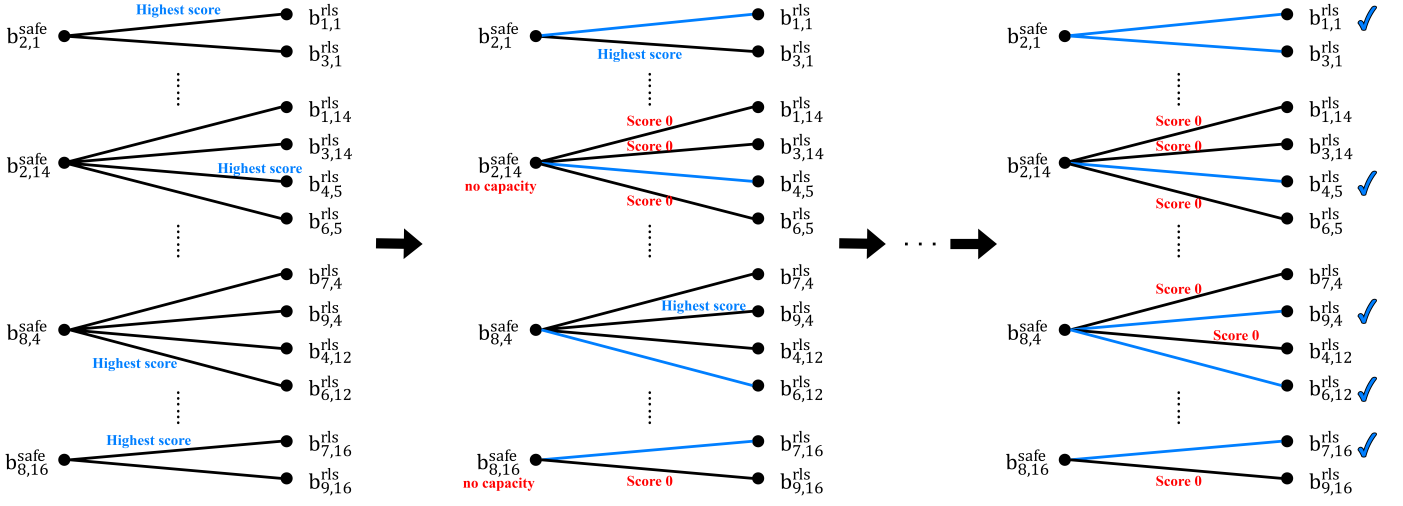
Fig. 7. Example of iterative edge activation and graph update in SBR.
