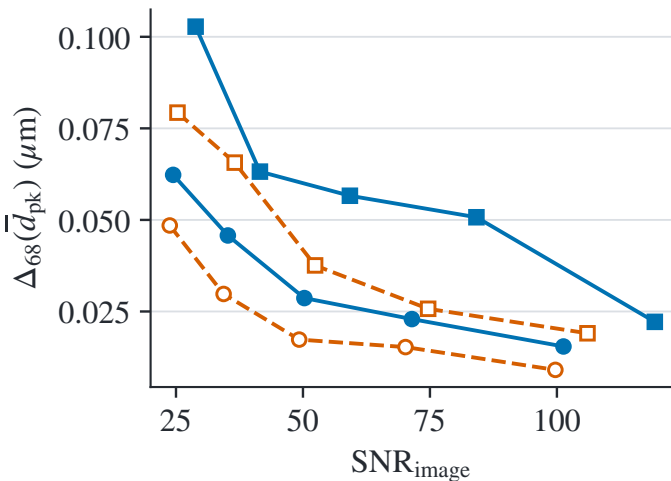
(c) SSP/ID peak separation
