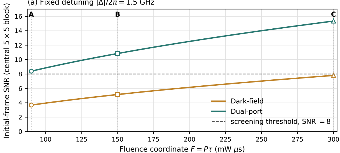
(a) Fixed detuning |\Delta|/2\pi = 1.5 GHz
