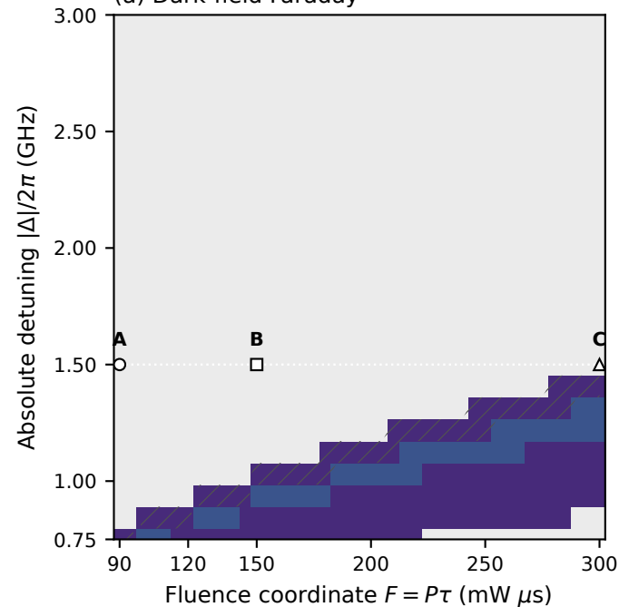
(a) Dark-field Faraday
