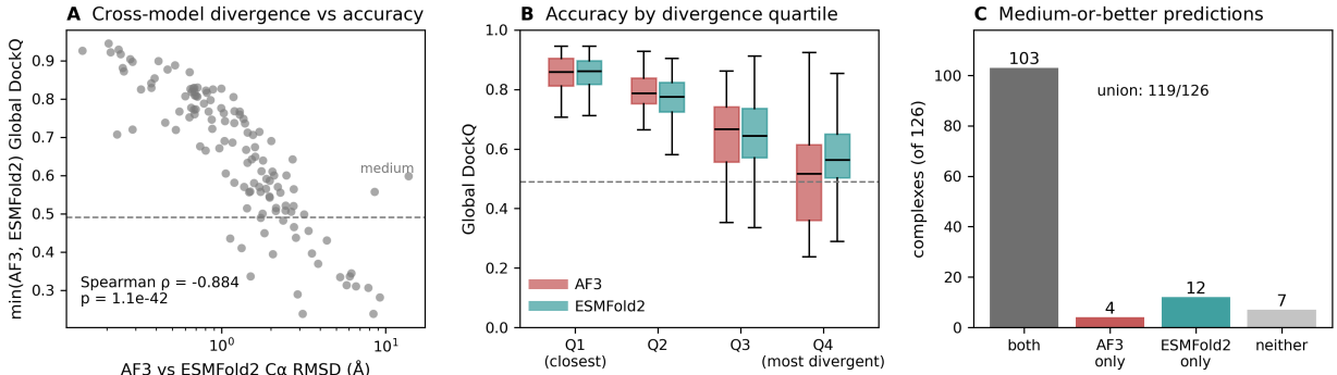
Figure 7: Structural divergence between the AlphaFold 3 and ESMFold2 predictions. (A) C \alpha RMSD between the AlphaFold 3 and ESMFold2 predictions of the same sequence against the worse of their two Global DockQ scores. (B) Global DockQ by quartile of that divergence; the two methods degrade together. (C) Complexes reaching medium-or-better accuracy: individually, jointly, and neither.
