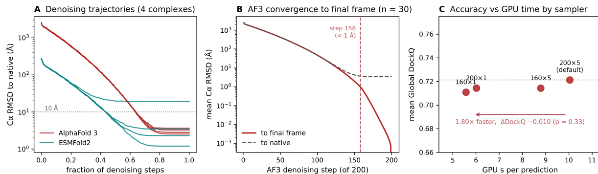
Figure 9: Denoising trajectories and AlphaFold 3 sampler economy. (A) C\alpha RMSD to the native along the denoising trajectory for four complexes traced in both models; AlphaFold 3 (200 steps, initial \sigma \approx 2,560 Å) is still tens of ångströms out at its midpoint, ESMFold2 (68 recorded steps, initial \sigma \approx 256 Å) is within a few ångströms. (B) AlphaFold 3 convergence to its own final frame over 30 complexes \times 5 samples; band spans median to 90th percentile. (C) GPU time against mean Global DockQ for four sampler configurations on the same 30 complexes.
