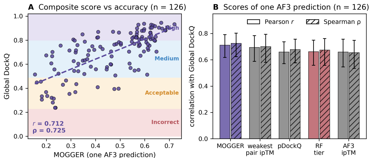
Figure 4: A composite single-prediction score against the published alternatives. (A) Global DockQ against MOGGER for the 126 complexes, with the linear fit and both correlations; shaded bands are the CAPRI quality classes. (B) Correlation with Global DockQ for every score computable from one AlphaFold 3 prediction, over all 126 complexes; whiskers are 95% bootstrap intervals.
