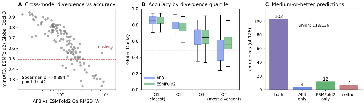
Figure 5: Structural divergence between the AlphaFold 3 and ESMFold2 predictions. (A) Cα RMSD between the AlphaFold 3 and ESMFold2 predictions of the same sequence against the worse of their two Global DockQ scores. (B) Global DockQ by quartile of that divergence; the two methods degrade together. (C) Complexes reaching medium-or-better accuracy: individually, jointly, and neither.
