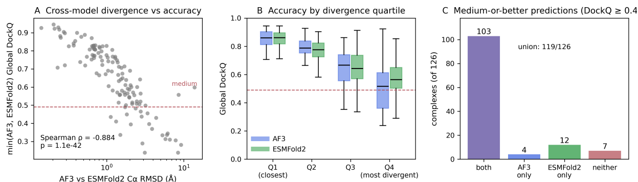
Figure 3: Structural divergence between the AlphaFold 3 and ESMFold2 predictions. (A) Cα RMSD between the AlphaFold 3 and ESMFold2 predictions of the same sequence against the worse of their two Global DockQ scores. (B) Global DockQ by quartile of that divergence; the two methods degrade together. (C) Complexes reaching medium-or-better accuracy: individually, jointly, and neither.
