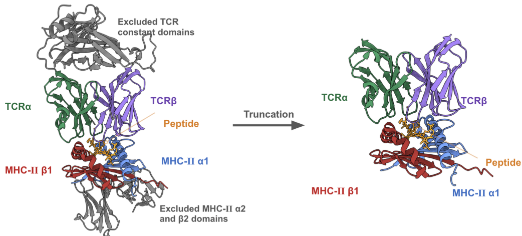
Figure 1: Domain truncation applied to the benchmark complexes. (A) Class I. The TCR constant domains, the MHC \alpha 3 domain and \beta 2-microglobulin are removed, leaving the MHC-I \alpha 1 \alpha 2 peptide-binding platform, the peptide and the paired TCR variable domains. (B) Class II. The TCR constant domains and the MHC-II \alpha 2 and \beta 2 domains are removed, leaving the \alpha 1 and \beta 1 peptide-binding domains, the peptide and the paired TCR variable domains. Retained chains are coloured by role; removed regions are grey.
