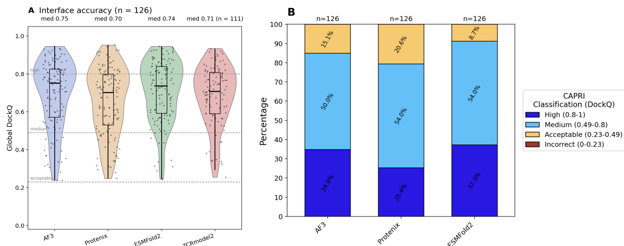
Figure 1: Interface accuracy on 126 post-cutoff TCR-pMHC complexes. (A) Distribution of Global DockQ per method; box, IQR and median; dots, individual complexes; dashed lines, CAPRI thresholds. TCRmodel2 covers the 111 class I complexes only. (B) The same data as CAPRI classes. No method produced an incorrect model of any complex.
