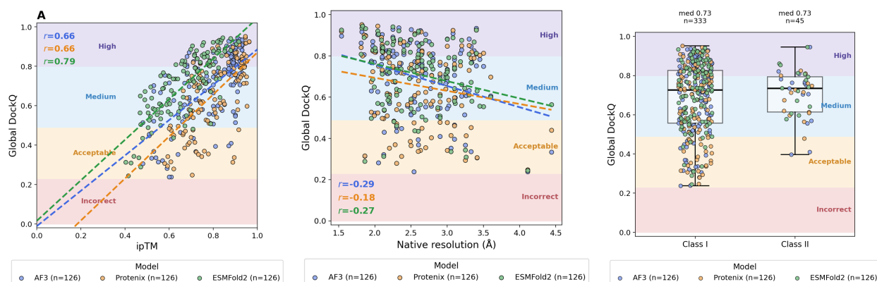
Figure 2: Determinants of interface accuracy. (A) Global DockQ against each method’s own ipTM, with per-method linear fits and Pearson r . ESMFold2’s confidence is both more conservative — it reaches a given DockQ at a lower ipTM — and better ordered. (B) Global DockQ against the resolution of the experimental reference. (C) Global DockQ by MHC class. Shaded bands are the CAPRI quality classes.
