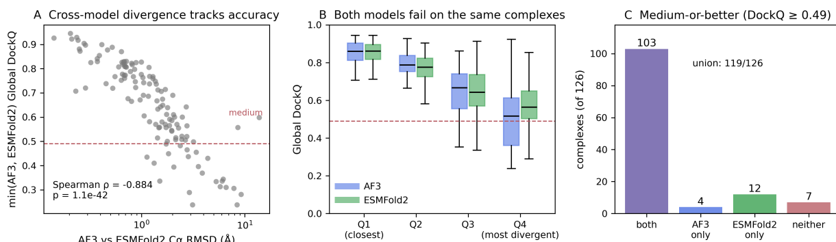
Figure 3: Cross-architecture disagreement is a reference-free accuracy signal. (A) Cα RMSD between the AlphaFold 3 and ESMFold2 predictions of the same sequence against the worse of their two Global DockQ scores. (B) Global DockQ by quartile of that divergence; the two methods degrade together. (C) Complexes reaching medium-or-better accuracy: individually, jointly, and neither.
