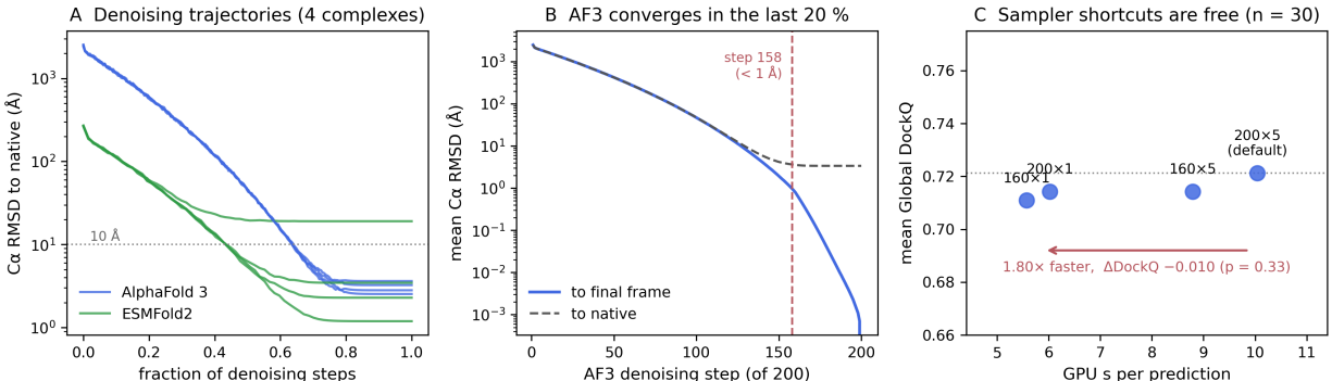
Figure 4: Both samplers reach the answer, by different routes, and earlier than the schedule assumes. (A) Cα RMSD to the native along the denoising trajectory for four complexes traced in both models; AlphaFold 3 (200 steps, initial \sigma \approx 2,560 Å) is still tens of ångströms out at its midpoint, ESMFold2 (68 recorded steps, initial \sigma \approx 256 Å) is within a few ångströms. (B) AlphaFold 3 convergence to its own final frame over 30 complexes \times 5 samples; band spans median to 90th percentile. (C) GPU time against mean Global DockQ for four sampler configurations on the same 30 complexes.
