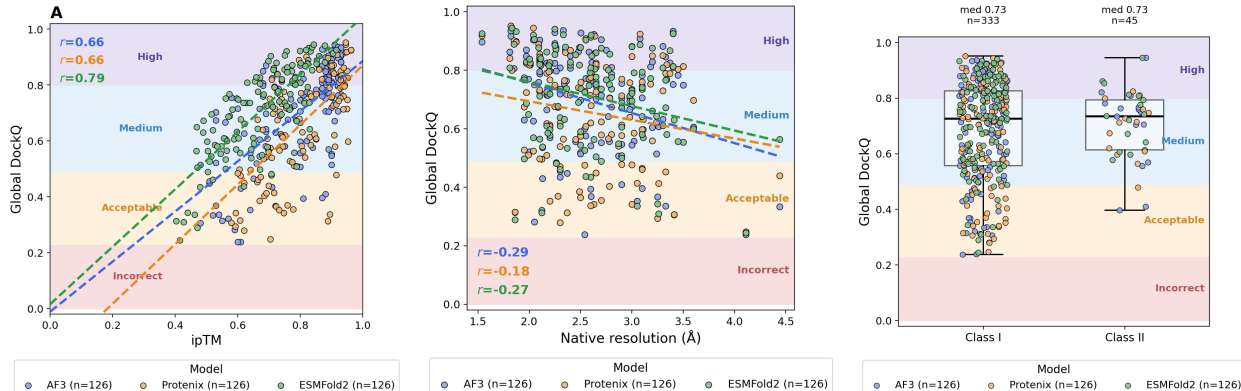
Figure 3: Determinants of interface accuracy. (A) Global DockQ against each method’s own ipTM, with per-method linear fits and Pearson r . ESMFold2’s confidence is both more conservative — it reaches a given DockQ at a lower ipTM — and better ordered. (B) Global DockQ against the resolution of the experimental reference. (C) Global DockQ by MHC class. Shaded bands are the CAPRI quality classes.
