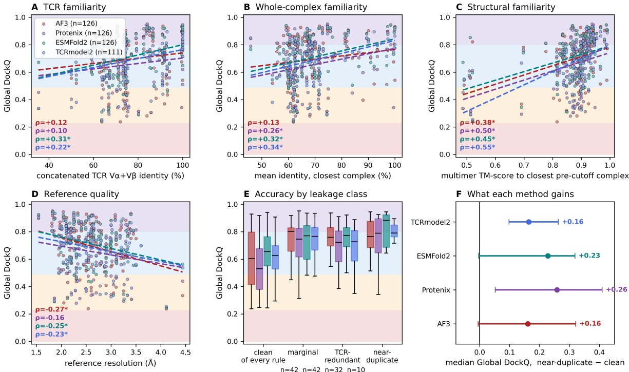
Figure 5: What accuracy tracks besides the model. (A) Global DockQ against concatenated TCR Vα+Vβ identity to the closest pre-cutoff complex, (B) against mean identity across all chains of the closest complex, (C) against the multimer TM-score between the target’s own experimental structure and the closest pre-cutoff complex, and (D) against the resolution of the experimental reference; dashed lines are per-method linear fits and \rho is Spearman, starred where p < 0.05 . (E) Accuracy by audit class. (F) Median Global DockQ gained on the 10 near-duplicates relative to the 42 targets clean of every criterion, with 95% bootstrap intervals. Shaded bands in A–E are the CAPRI quality classes.
