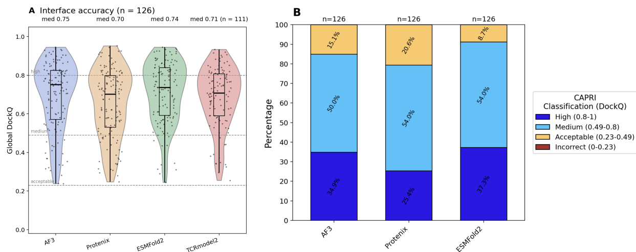
Figure 2: Interface accuracy on 126 post-cutoff TCR-pMHC complexes. (A) Distribution of Global DockQ per method; box, IQR and median; dots, individual complexes; dashed lines, CAPRI thresholds. TCRmodel2 covers the 111 class I complexes only. (B) The same data as CAPRI classes. No method produced an incorrect model of any complex.
