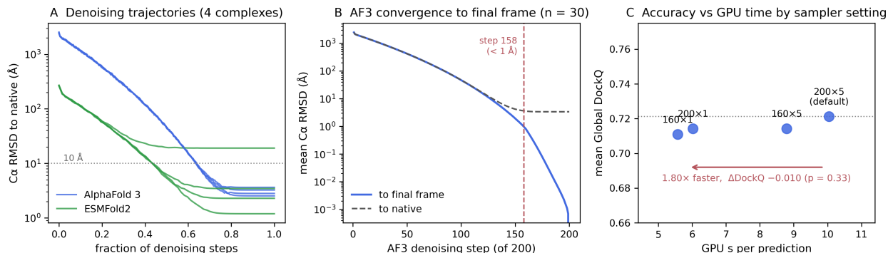
Figure 5: Denoising trajectories and AlphaFold 3 sampler economy. (A) Cα RMSD to the native along the denoising trajectory for four complexes traced in both models; AlphaFold 3 (200 steps, initial \sigma \approx 2,560 Å) is still tens of ångströms out at its midpoint, ESMFold2 (68 recorded steps, initial \sigma \approx 256 Å) is within a few ångströms. (B) AlphaFold 3 convergence to its own final frame over 30 complexes \times 5 samples; band spans median to 90th percentile. (C) GPU time against mean Global DockQ for four sampler configurations on the same 30 complexes.
