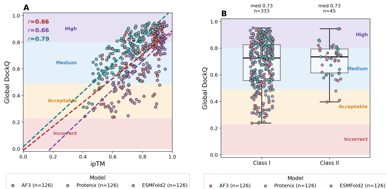
Figure 4: Determinants of interface accuracy. (A) Global DockQ against each method’s own ipTM, with per-method linear fits and Pearson r . ESMFold2’s confidence is both more conservative, reaching a given DockQ at a lower ipTM, and better ordered. (B) Global DockQ by MHC class. Shaded bands are the CAPRI quality classes.
